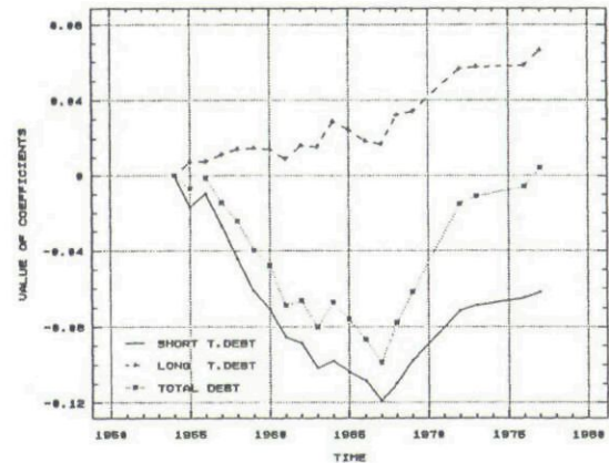
Fig. 2. Coefficients of time dummies
