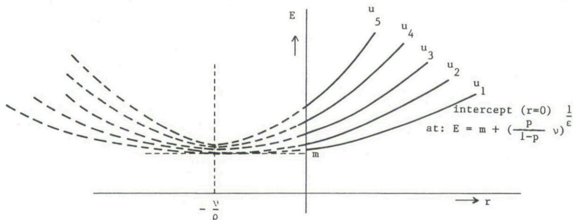
Fig. 4. Indifference curves.
