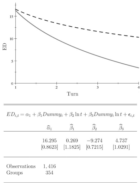
Figure 4 Convergence of estimates' dispersion across turns The figure depicts the convergence rate of estimates' dispersion across turns in the BLT (solid line) and OCT (dashed line). The rates are obtained from estimating the model ED_{i,t} = \alpha_1 + \beta_1 Dummy_i + \beta_2 \ln t + \beta_3 Dummy_i \ln t + \epsilon_{i,t} , treating the data as a panel (market instances and turns). ED_{i,t} is the estimates' dispersion in turn t of observation i , Dummy_i takes the value 1 if observation i is obtained in the OCT and 0 otherwise, and t is the turn number. Robust standard errors are reported in square brackets.
