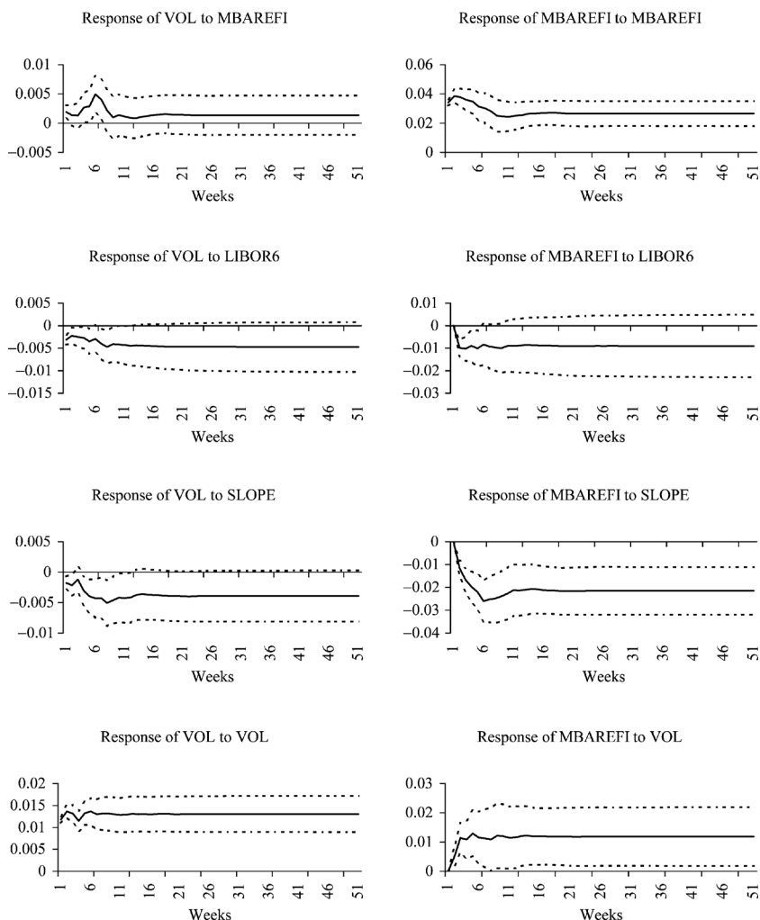
Figure 3 Impulse response functions.
