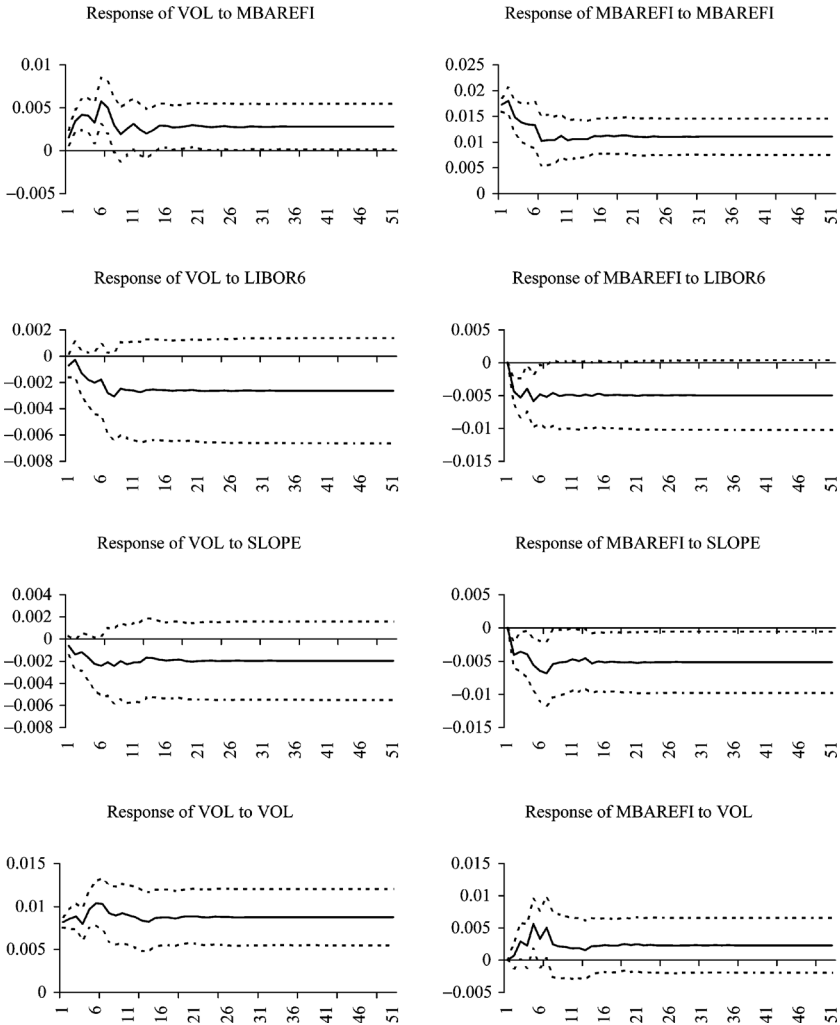
Figure 4 Impulse response functions estimated using data through December 2000.
