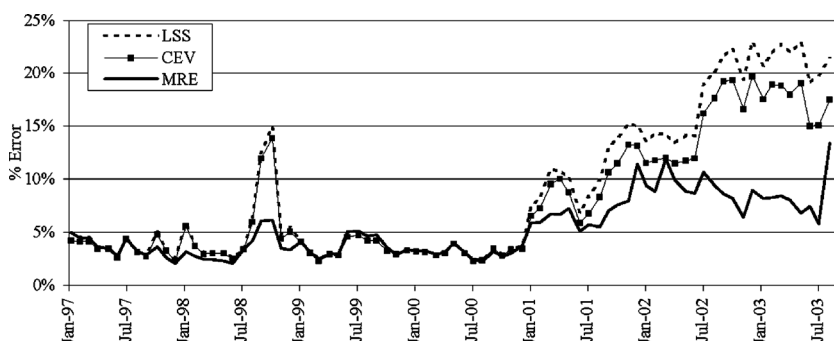
Figure 5 RMSE of each calibrated model.
