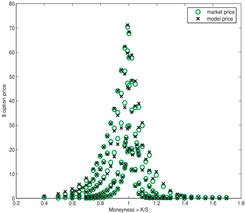
Figure 2 Calibration of the GJR GARCH model with the FHS method on the cross-section of out-of-the-money SPX options on 9 July 2003.
