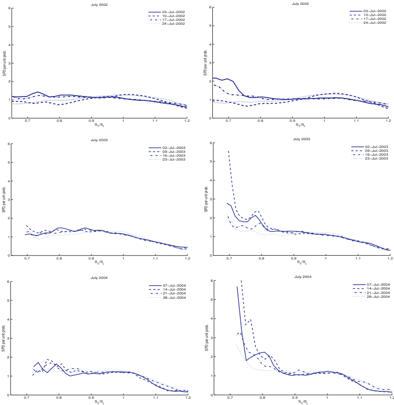
Figure 7 SPD per unit probability on four consecutive Wednesdays in July 2002, July 2003, and July 2004 and for time to maturity \tau closest to 100 days. SPD per unit probability, M_{t,t+\tau} , is estimated by the discounted ratio of the pricing over the historical densities. For each Wednesday t , the pricing GJR model is calibrated on the cross-section of out-of-the-money SPX options, and the historical GJR model is estimated using 3,500 historical S&P 500 log-returns. Two estimates of M_{t,t+\tau} are provided using (i) the FHS method (left graphs) and (ii) the GAUSS method (right graphs). In case (i), historical and pricing GJR models are simulated using FHS innovations, and in case (ii), using Gaussian innovations.
