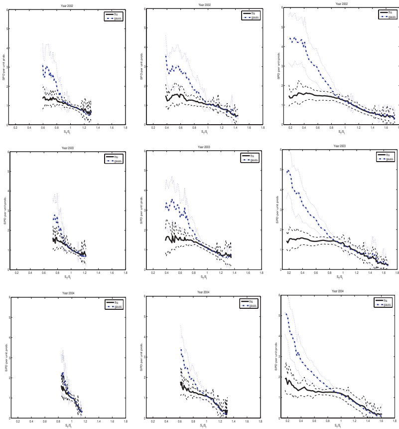
Figure 6 Average SPD per unit probability for 2002, 2003, and 2004 (from top to bottom), and short, medium, and long maturities (from left to right).
