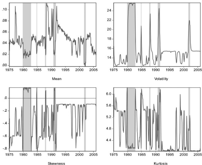
Figure 3 Mean excess returns, volatility, skewness, and kurtosis of the world market portfolio implied by the two-state model (annualized figures). Periods where the global bear state is most likely are shown in gray shades.
