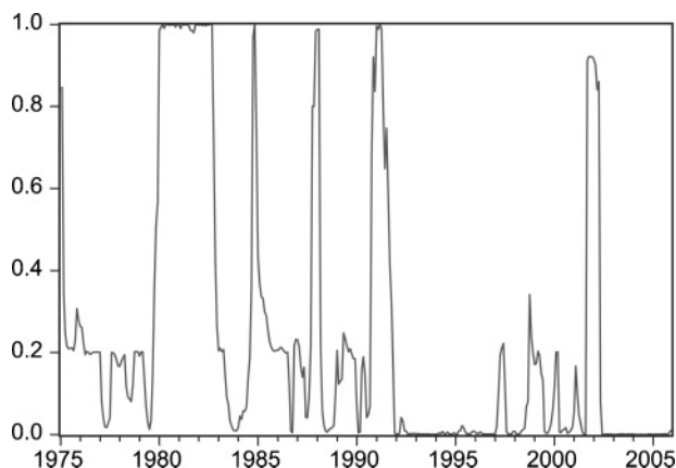
Figure 1 Bear state probabilities.
