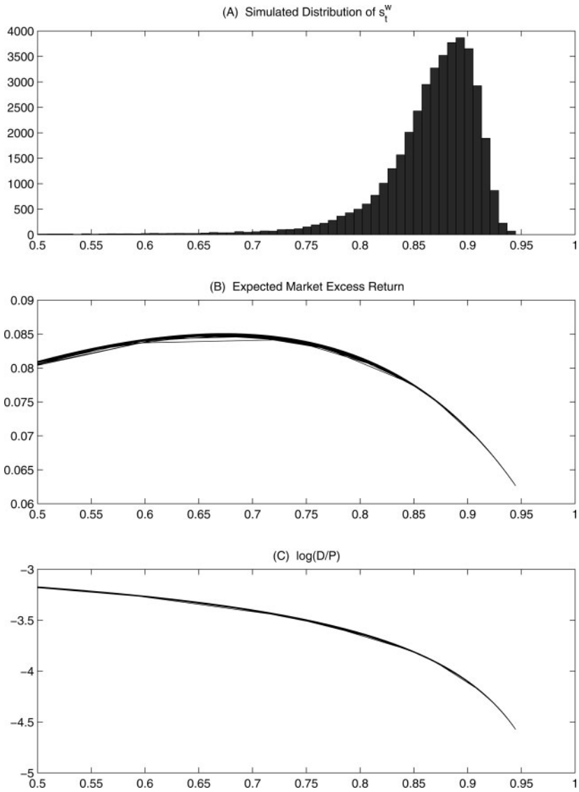
Figure 3 Simulations Panel A: histogram of simulated share s_t^w = w_t/C_t (see notes to Table 4 for details on simulation). Panel B: theoretical expected return plotted against the labor income share s_t^w . Panel C: model implied log dividend-price ratio as a function of labor income share s_t^w .
