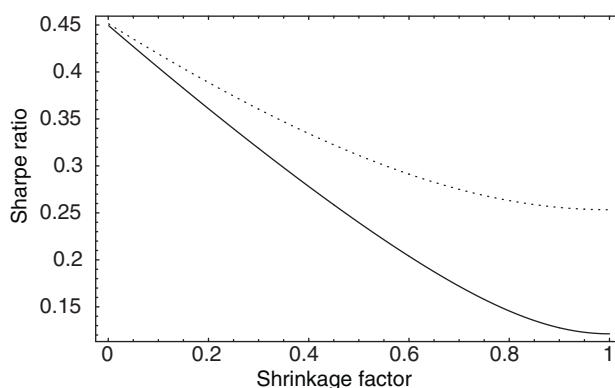
Figure 1 Optimal Sharpe ratio as a function of the shrinkage factor
