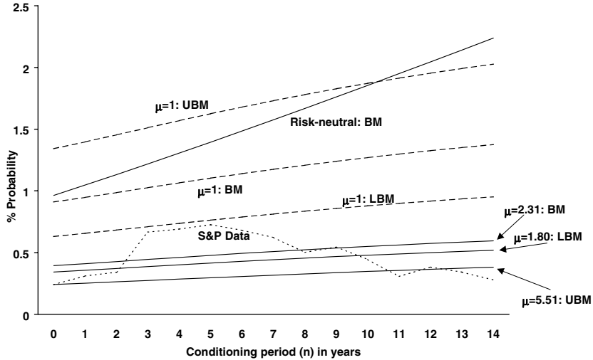
Figure 3 Conditional default probabilities
