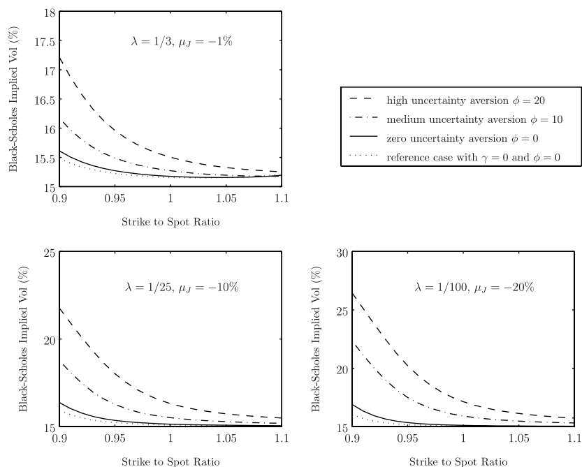
Figure 1 The equilibrium “smile” curves
