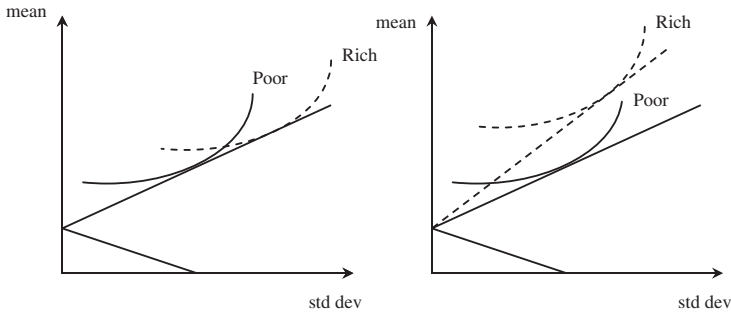
Figure 6 Efficient frontier and investors' portfolio choice in the risk aversion model (left panel) and the information model (right panel) The figure displays utility curves and mean-variance frontiers for two investors with different levels of initial wealth.
