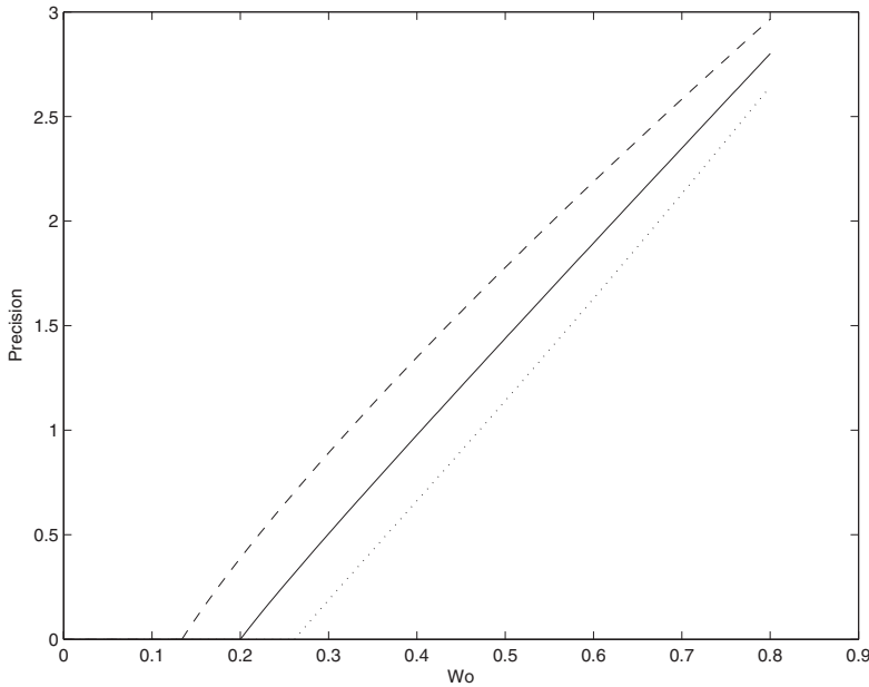
Figure 3 The optimal precision for different levels of wealth under constant (solid curve) decreasing (dotted curve), and increasing (dashed curve) relative risk aversion
