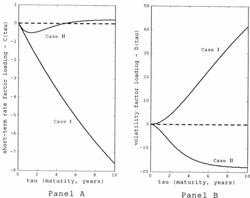
Figure 2 Factor loadings for Equations (10)
