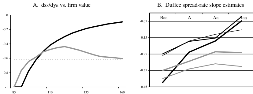
Figure 6 Theoretical and empirical slopes of the spread-rate relation
