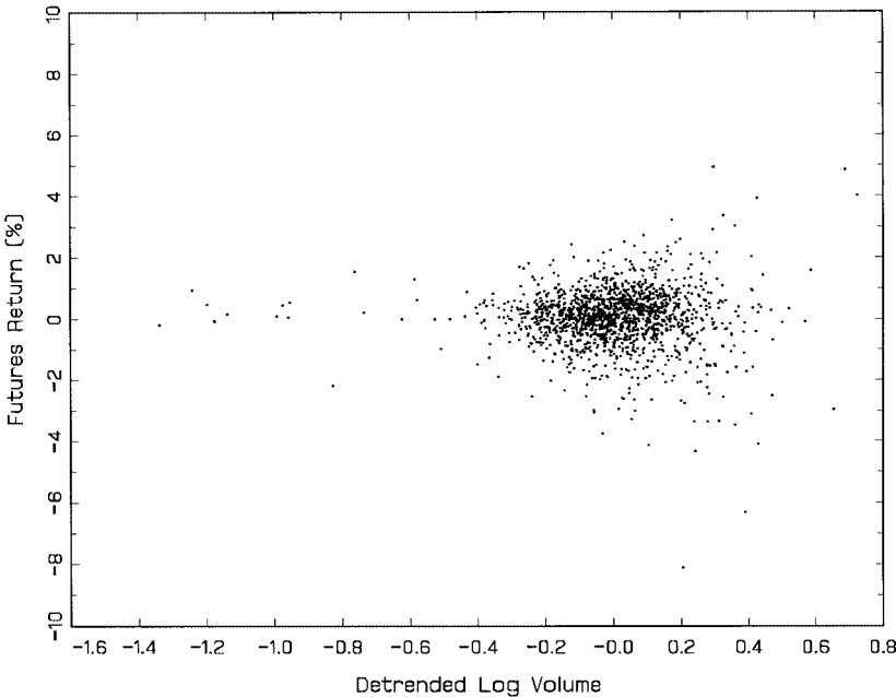
Figure 5 A scatter plot of detrended log trading volume ( \ln(1 + vol_t^S) ) in the U.S. spot market and the futures return ( r_t^F ) on the Russell 2000.
