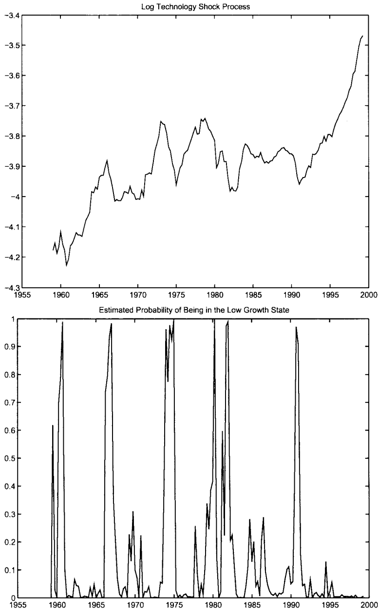
Figure 1 The top panel displays the logarithm of the technology level (the cumulation of the Solow residual) and the bottom panel displays the probability of being in the low-growth state.
