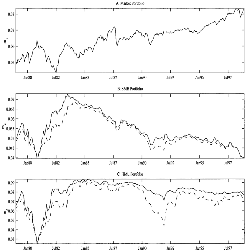
Figure 3 Plots of the time series of the posterior asset drift parameters under the two different priors for (A) market, (B) SMB, and (C) HML portfolios
