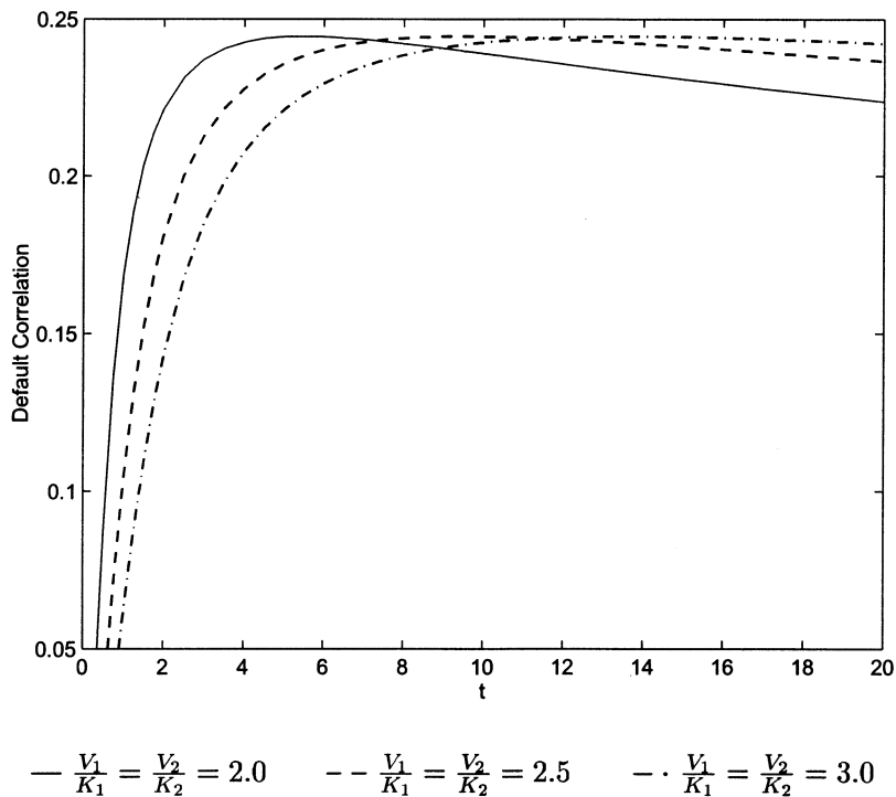
Figure 2 The relation between default correlation and time for various credit qualities Here \rho represents the asset level correlation between firms and t is the length of time horizon. The parameter values used here are \rho = 0.4 and \sigma_1 = \sigma_2 = 0.4 .
