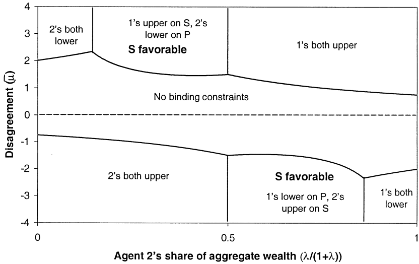
Figure 2 Equilibrium regions in the case of two-sided constraints on both risky securities (Section 5)
