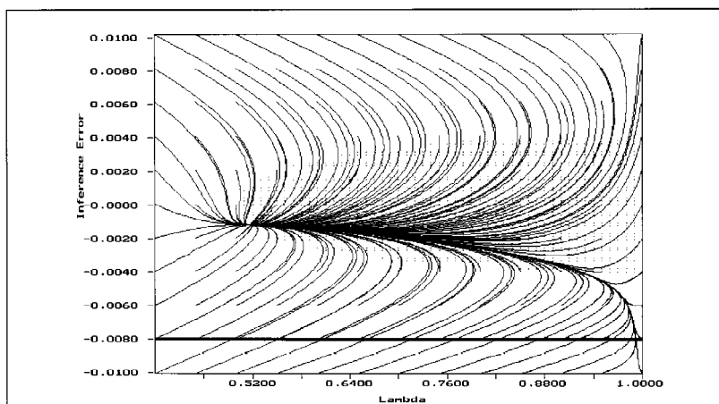
Figure 4 Phase plots in learning process with drift Each line represents a different initial condition. Note that all lines converge to a point which is close to the GS equilibrium.
