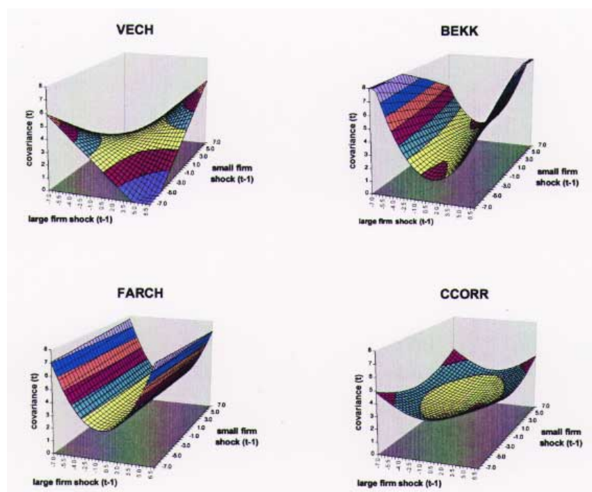
Figure 1 News impact surfaces for covariances The figures give the news impact surfaces for the covariance between small-firm and large-firm return shocks under the Vech model, the BEKK model, the FARCH model, and the CCORR model.
