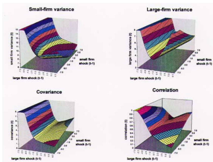
Figure 5 News impact surfaces for ADC model
