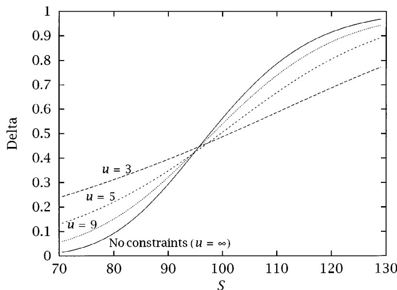
Figure 2 Standard call option Illustration of \Delta(S) for several values of u . The option parameters are K = 100 , r = 0.05 , \sigma = 0.3 , and T = 0.25 .
