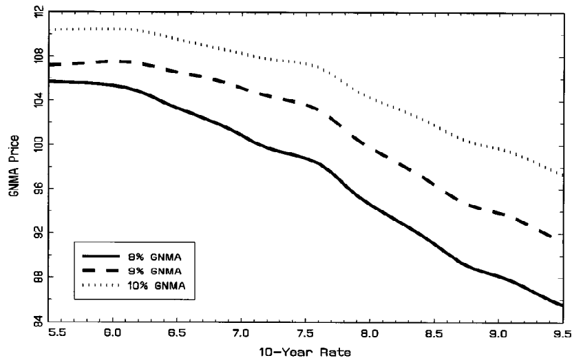
Figure 9 Estimated GNMA prices and interest rates
