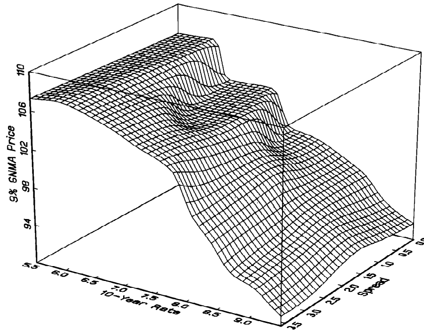
Figure 7 GNMA estimated (two-factor) prices
