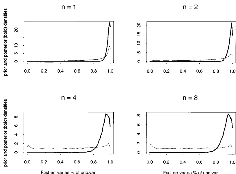
Figure 4 Prior and posterior densities for forecastability as a function of the size of the conditioning set
