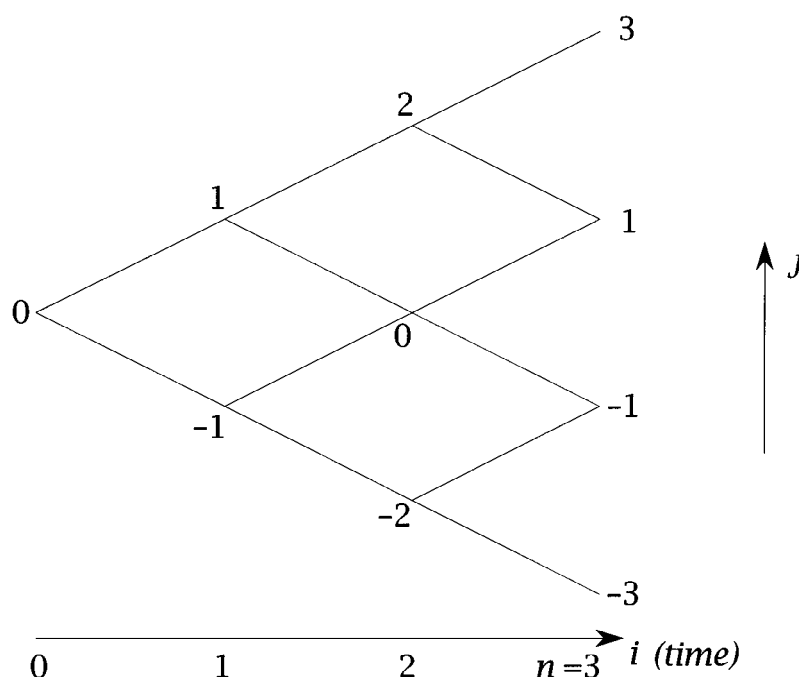
Figure 10 Illustration of the binomial tree for n = 3 Time is indexed i = 0, \dots, n . At time i , asset prices are indexed by j = -i, -i + 2, \dots, i - 2, i .
