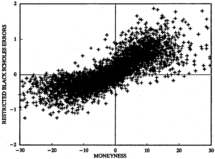
Figure 2 Pricing errors from the restricted Black-Scholes model graphed against the moneyness of the option.
