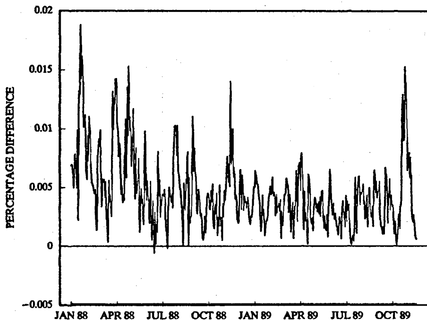
Figure 1 Percentage difference between the implied value of the index and the actual market value of the index The implied value of the index is obtained by inverting the Black-Scholes model using daily sets of simultaneous S&P 100 index call option prices.
