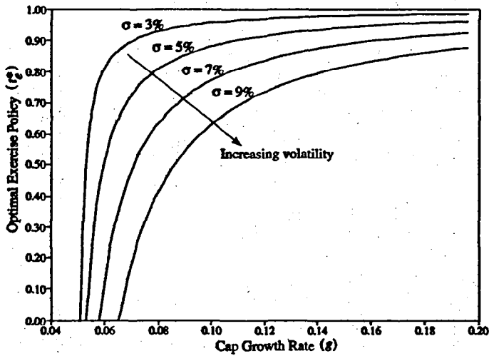
Figure 5 Optimal exercise policy vs. cap growth rate
