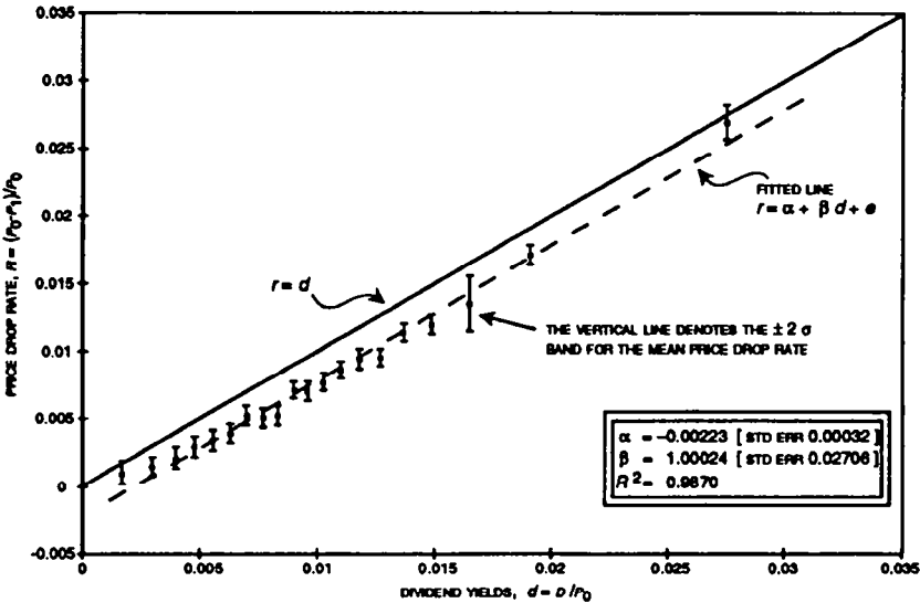
Figure 3 The linear relation between price drop rate and dividend yield
