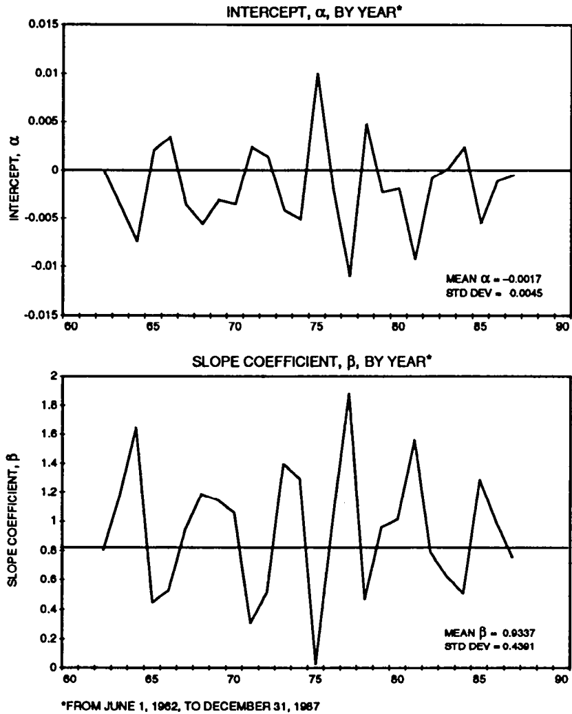
Figure 4 Stability over time of the intercept ( \alpha ) and slope ( \beta ) coefficients in the linear relation between price drop and dividend yield
