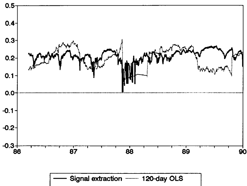
Figure 3 Comparison of signal extraction and 120-day OLS regression coefficients for the model of SPD and NKN Comparison of signal extraction and 120-day OLS regression coefficients for the model of SPD and NKN from April 1986 to December 1989. The solid line plots the estimated signal extraction coefficients reported in Table 6, while the broken line plots the estimated coefficients for the 120-day rolling regression of SPD on NKN
