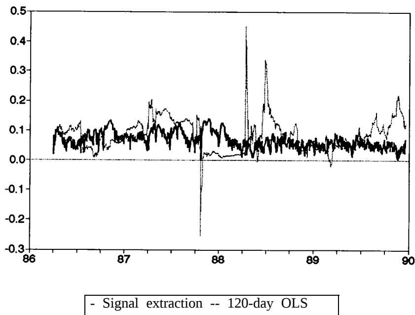
Figure 2 Comparison of signal extraction and 120-day OLS regression coefficients for the model of NKD and SPN
