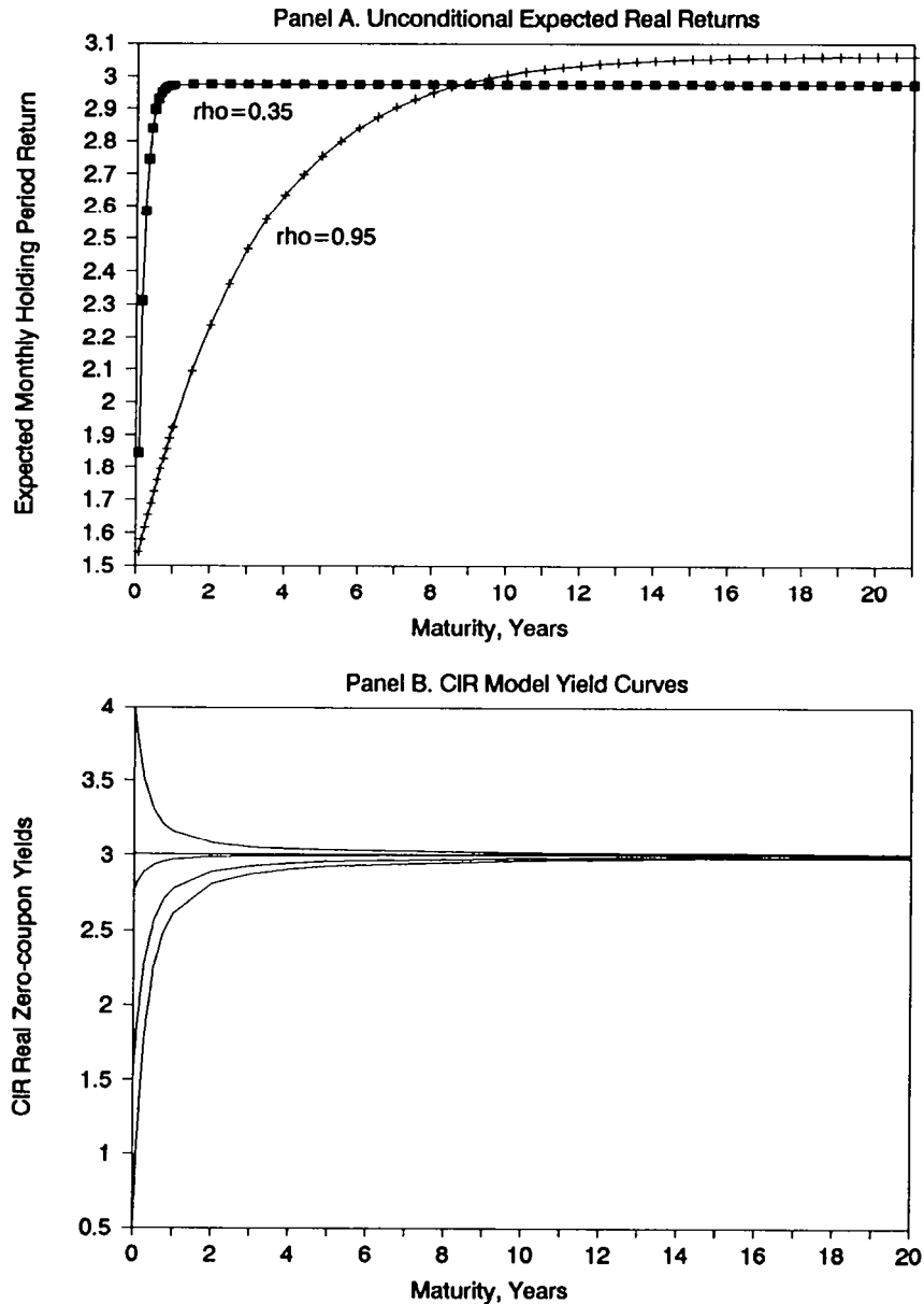
Figure 2 Expected returns and yields to maturity for the CIR model, using GMM parameter estimates. The parameter values used in both figures are \theta = 1.54 percent, \rho = 0.35 , y_{\infty} := 3.01 percent, and \sigma_u := 1.23 percent. Panel A shows the annualized expected monthly holding period returns for indexed bonds of various maturities for two values of the autocorrelation coefficient: \rho = 0.35 (the fitted estimate) and \rho = 0.95 . Panel B shows yield curves for the CIR model for each of five values of the instantaneous rate r = 4.00, 3.00, 2.77, 1.54 , and 0.50 percent.
