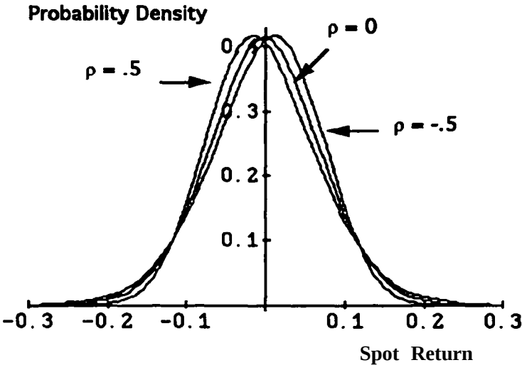
Figure 1 Condition probability density of the continuously compounded spot return over a six-month horizon Spot-asset dynamics are dS(t) = \mu S dt + \sqrt{v(t)} S dz_1(t) , where dv(t) = \kappa[\theta^* - v(t)]dt + \sigma\sqrt{v(t)} dz_2(t) . Except for the correlation \rho between z_1 and z_2 shown, parameter values are shown in Table 1. For comparison, the probability densities are normalized to have zero mean and unit variance.
