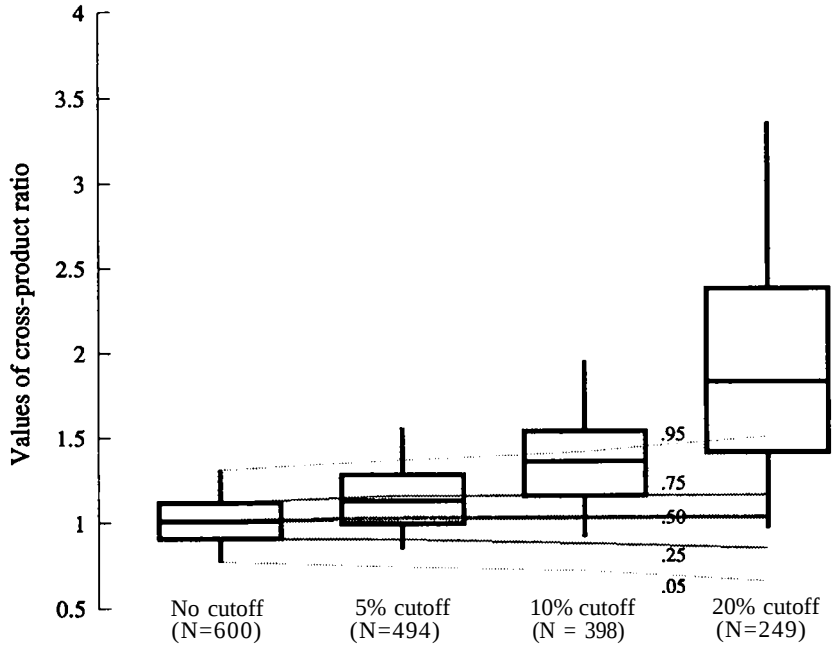
Figure 1 Boxplots of 20,000 simulated values of the cross-product ratio for different performance cutoff levels The solid line within each box represents the median of the empirical distribution of cross-product ratios, whereas the box itself gives the interquartile range. The whiskers above and below each box give the 95th and 5th percentiles, respectively, of the empirical distribution. The gray lines give the stated fractiles of the theoretical distribution implied by the hypergeometric distribution of cell counts assuming independence.
