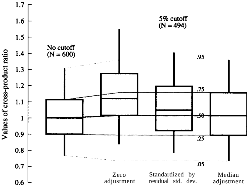
Figure 3 Boxplots of 20,000 simulated values of the cross-product ratio showing the effect of different adjustments for survivorship bias with a 5 percent performance cutoff Zero adjustment refers to the boxplot given in Figure 1, where there is a 5 percent performance cutoff. Standardized by the residual standard deviation refers to the cross-product ratio calculated on the basis of defining “winners” and “losers” relative to the median appraisal ratio. Median adjustment corrects the median for the fact that the distribution of appraisal ratios is truncated by survivorship. This correction is described in the text.
