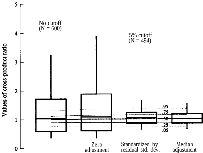
Figure 5 Boxplots of 20,000 simulated values of the cross-product ratio showing the effect of cross-correlation on alternative adjustments for survivorship bias
