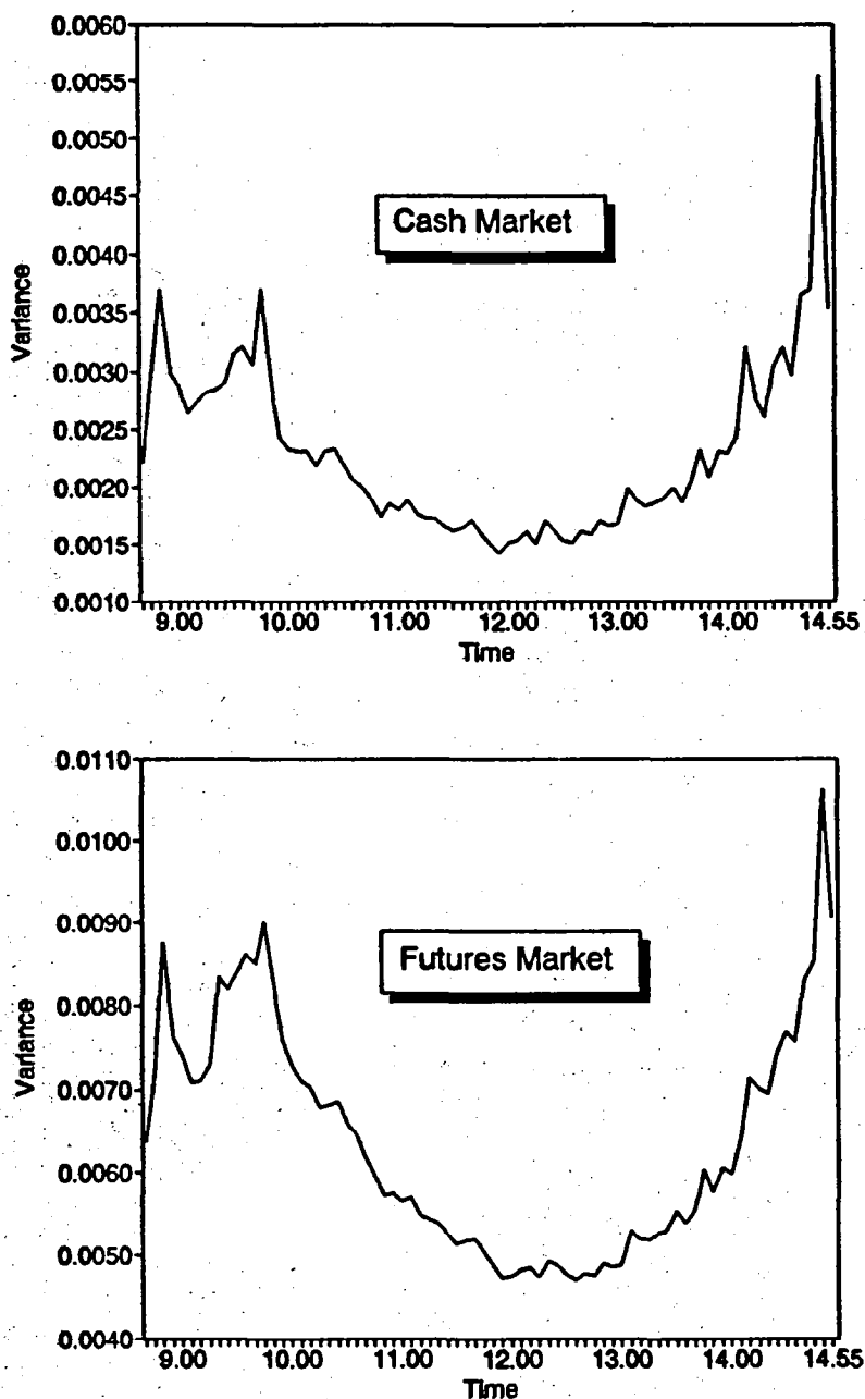
Figure 1 Intraday volatility of the S&P 500 stock index and S&P 500 stock index futures returns for November 1988–December 1989 Subperiod estimates for the bivariate AR(1)–GARCH(1,3) model with five-minute returns data are used to compute the conditional volatility series, which are then averaged over the number of days in the sample. “Time” is aligned to Central Time.
