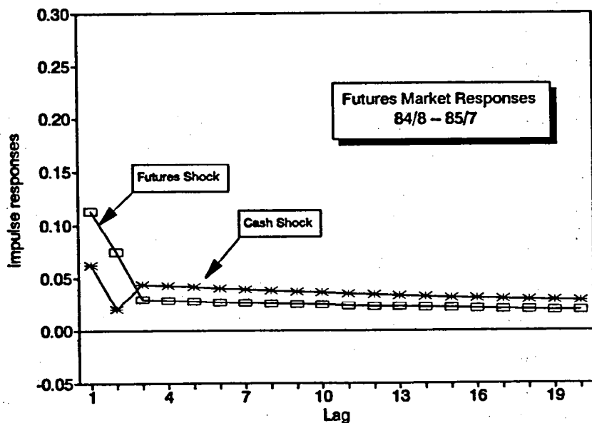
Figure 2 Impulse response functions of intraday conditional volatility of the S&P 500 stock index and S&P 500 stock index futures returns for August 1984–July 1985 Subperiod estimates for the bivariate AR(1)–GARCH(1,3) model with five-minute returns data are used to compute the impulse response coefficients following a unit return shock originating in each market.
