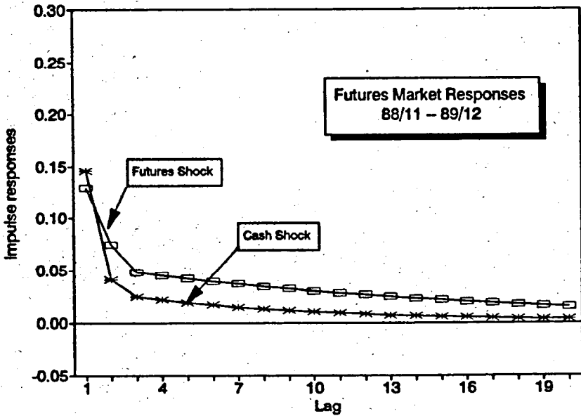
Figure 3 Impulse response functions of intraday conditional volatility of the S&P 500 stock index and S&P 500 stock index futures returns for November 1988–December 1989 Subperiod estimates for the bivariate AR(1)–GARCH(1,3) model with five-minute returns data are used to compute the impulse response coefficients following a unit return shock originating in each market.
