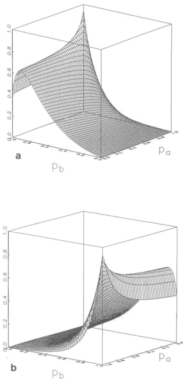
Figure 2 Cross-autocorrelation \rho_{10}^*(k) as a function of p_a and p_b , for q = 5 , k = 1 a: Front view; b: rear view.
