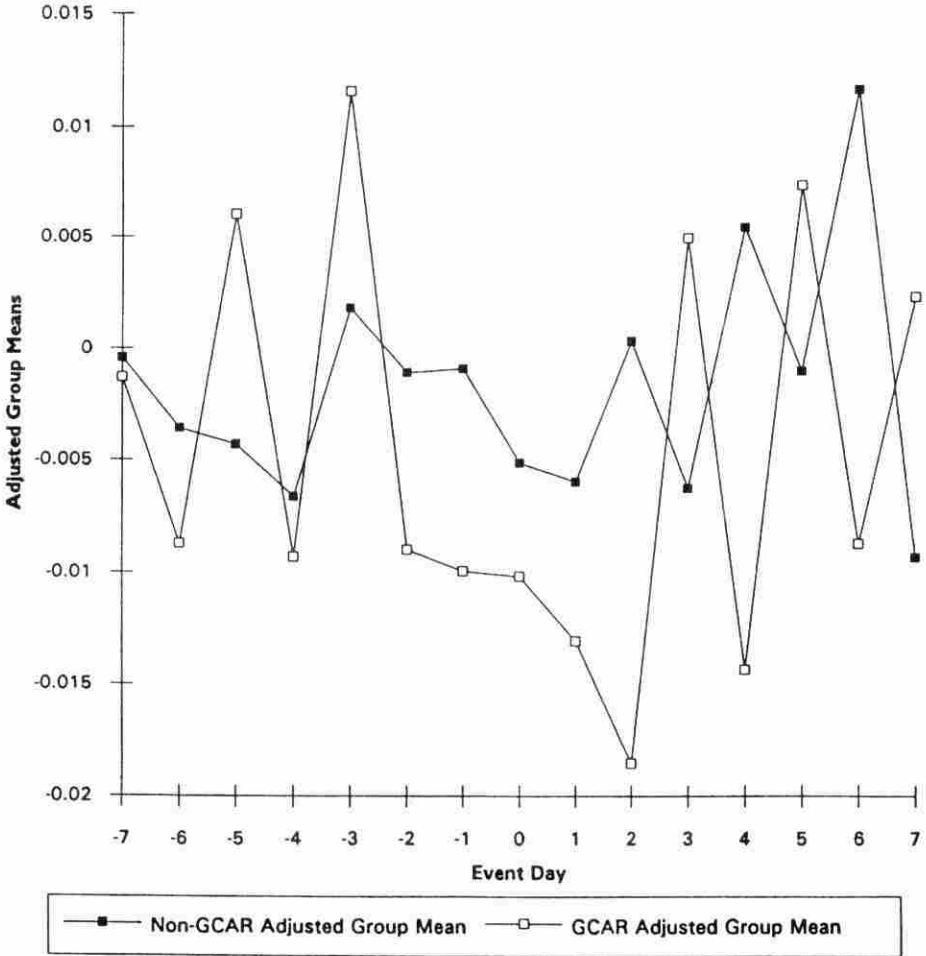
Figure 1-Plot of Adjusted Group Means for Event Period -7 Through +7 Days Surrounding Day Zero
