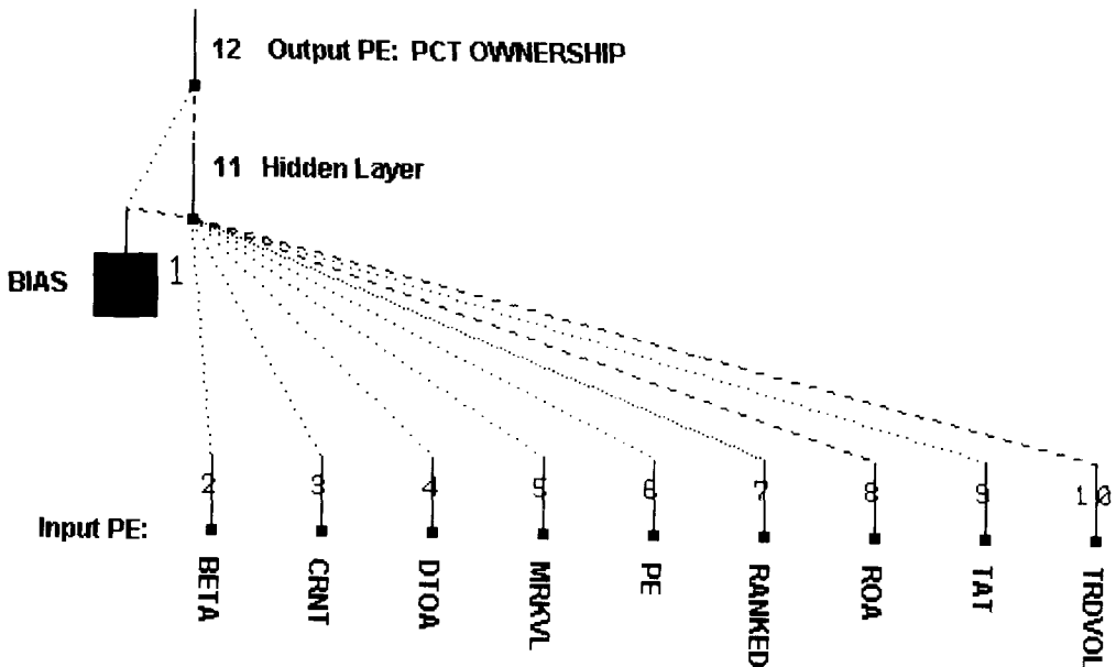
Figure 1—Neural Network Map
