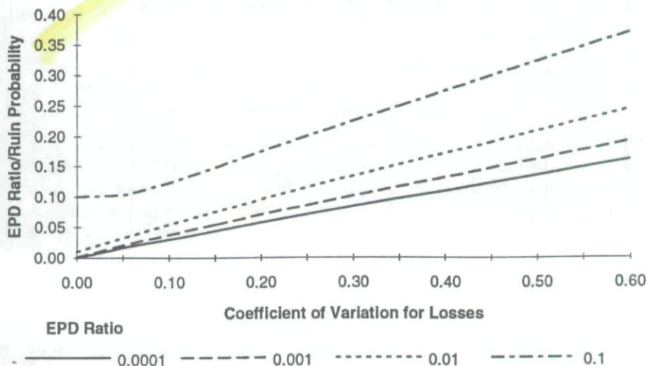
Figure 2 Expected Policyholder Deficit Ratio/Ruin Probability vs. Coefficient of Variation of Losses Under Normal Distribution
