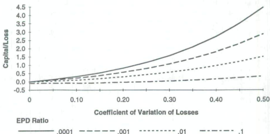
Figure 3 Capital/Loss vs. Expected Policyholder Deficit Ratio and Coefficient of Variation of Losses Under Lognormal Distribution
