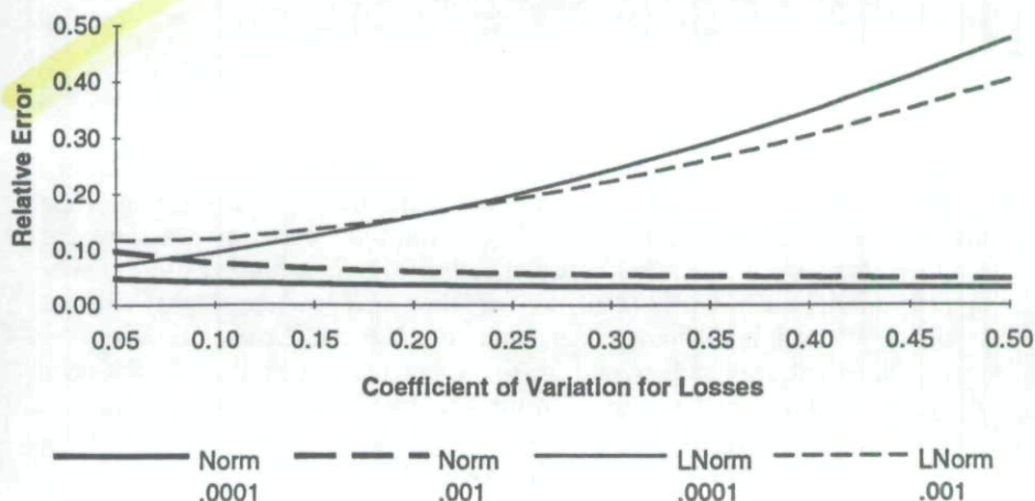
Figure 6 Relative Error Using Square Root Approximation for Losses Under Normal and Lognormal Distributions Expected Policyholder Deficit Ratios = 0.0001 and 0.001
