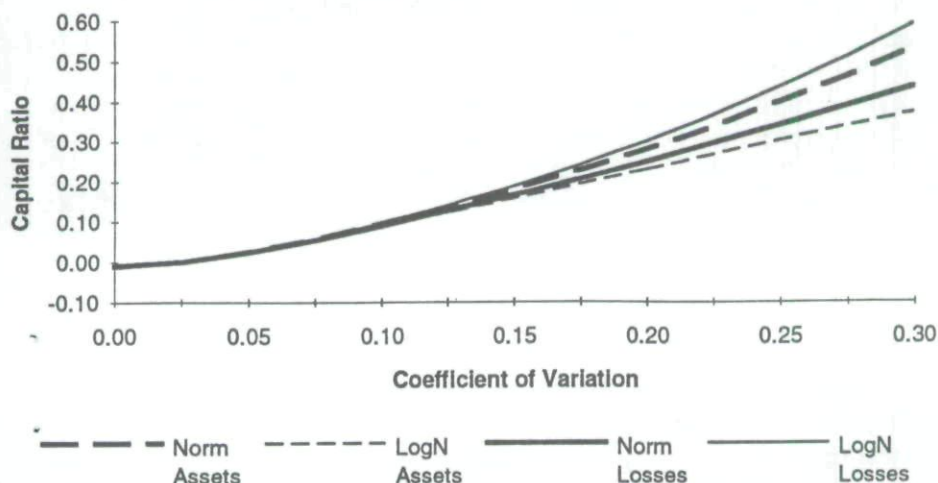
Figure 4 Comparison of Asset vs. Loss Capital Ratios for Normal and Lognormal Distributions Expected Policyholder Deficit Ratio = 0.01
