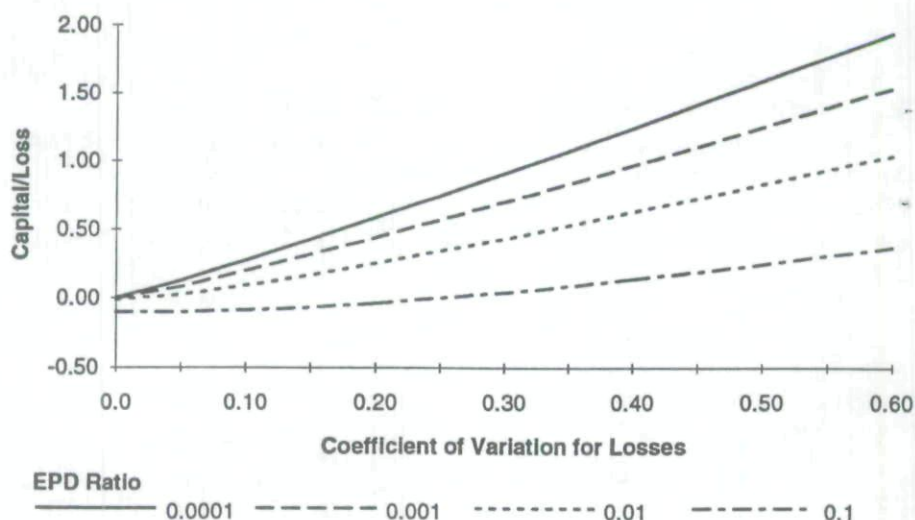
Figure 1 Capital/Loss vs. Expected Policyholder Deficit Ratio and Coefficient of Variation of Losses Under Normal Distribution
