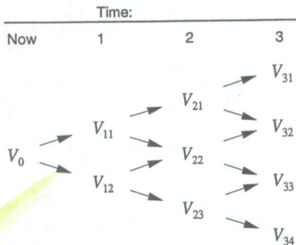
Figure 5 Time Dependence of Risk
