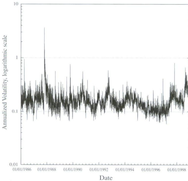
FIGURE 4 Annualized FTSE-100 volatility calculated each day from optimally weighted squared five-minute returns.
