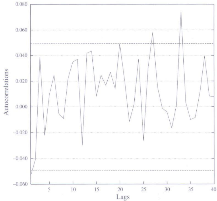
FIGURE 9 Autocorrelations of (1 - L)^{0.43}[\ln(\hat{\sigma}_t) - m_{j(t)}] .
