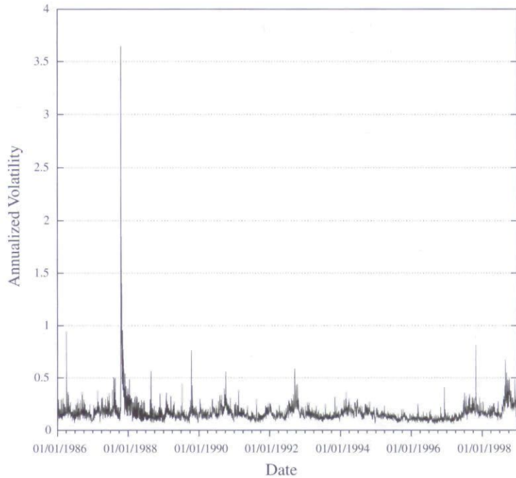
FIGURE 3 Annualized FTSE-100 volatility calculated each day from optimally weighted squared five-minute returns.
