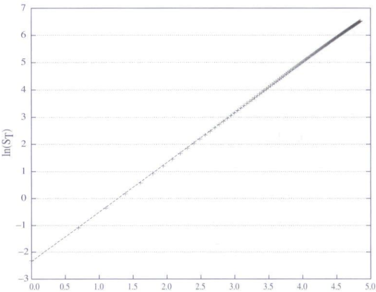
FIGURE 7 Scaling plot for daily logarithmic realized volatility, S_T is the variance of T consecutive observations.
