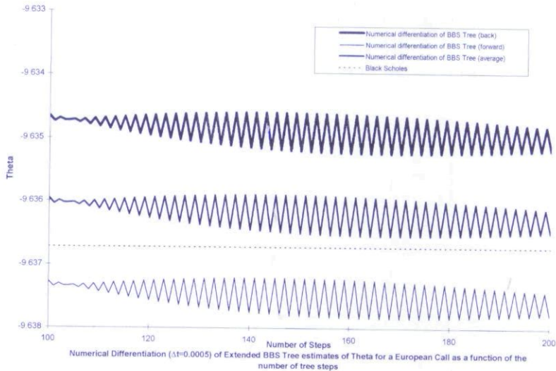
FIGURE 5 European Call Option \theta estimates.
