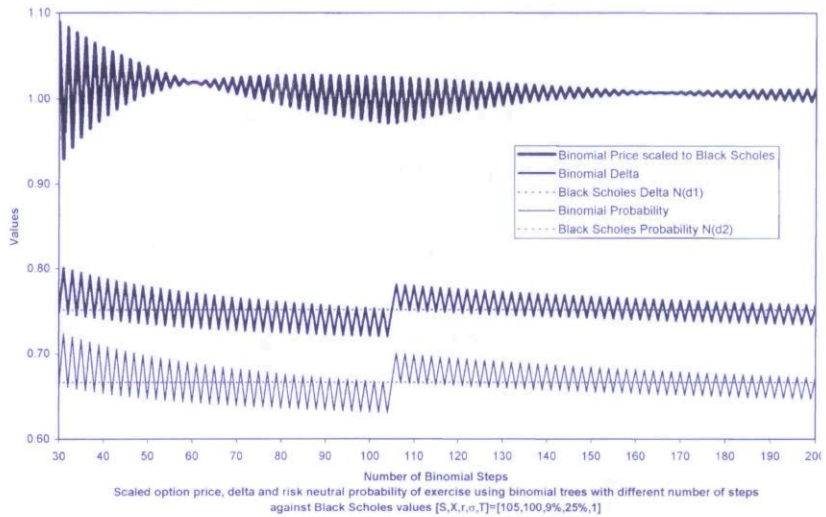
FIGURE 1 European (scaled) option pricing and Greeks.
