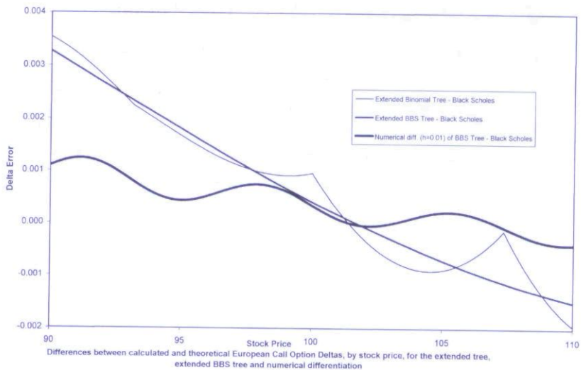
FIGURE 2 \Delta estimation error for a European Call Option.
