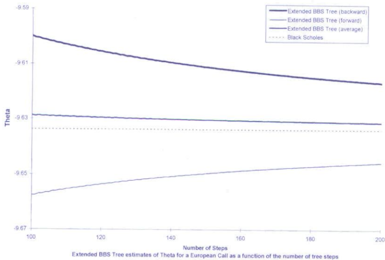
FIGURE 4 European Call Option \theta estimates.
