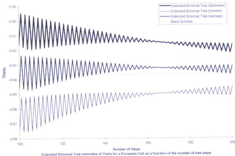
FIGURE 3 European Call Option \theta estimates.
