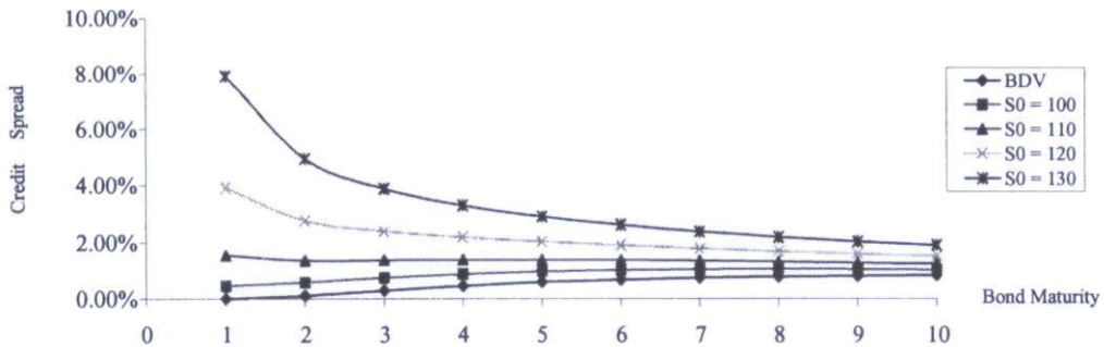
Credit Spread with \rho_{Ar} = 0.25
