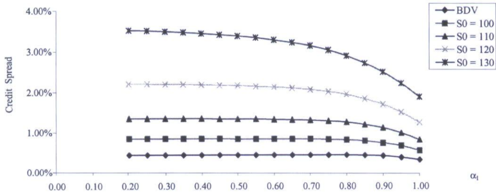
Effects of Changing \alpha_1 on Credit Spread
