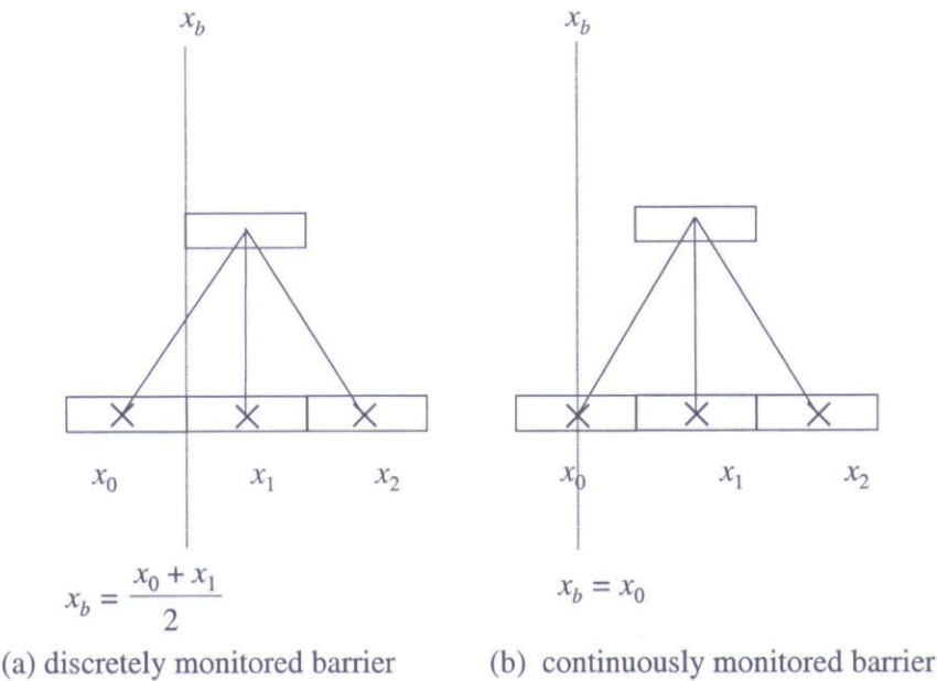
FIGURE 1 The different methods of placing the barrier node are shown for (a) discretely monitored barrier option, and (b) continuously monitored barrier option. To approximate the discretely monitored barrier condition with better accuracy, it is optimal to place the whole interval [x_0 - \frac{\Delta x}{2}, x_0 + \frac{\Delta x}{2}] to lie completely in the knockout region.
