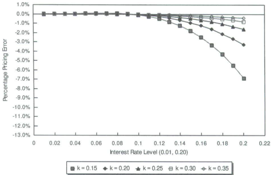
FIGURE 2 Pricing errors under different levels of mean reversion rate, k (CIR Model).
