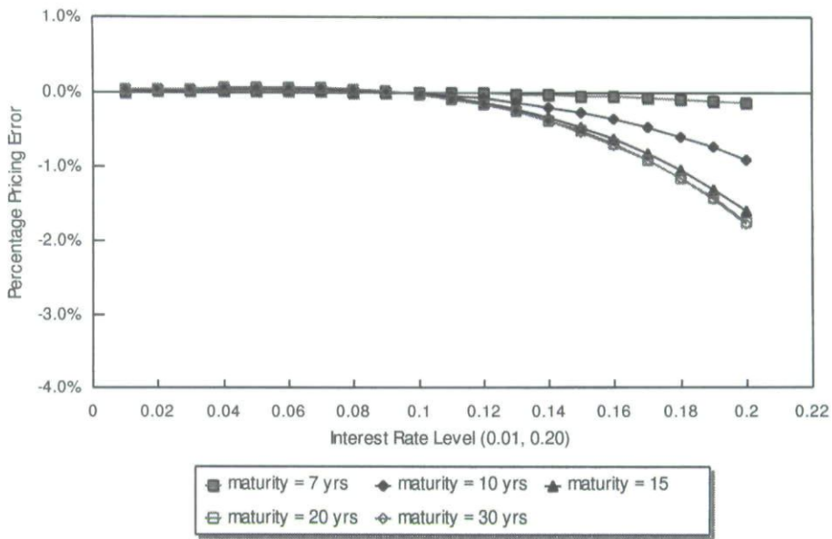
FIGURE 8 Pricing errors for options on bonds with different maturities (CIR Model).
