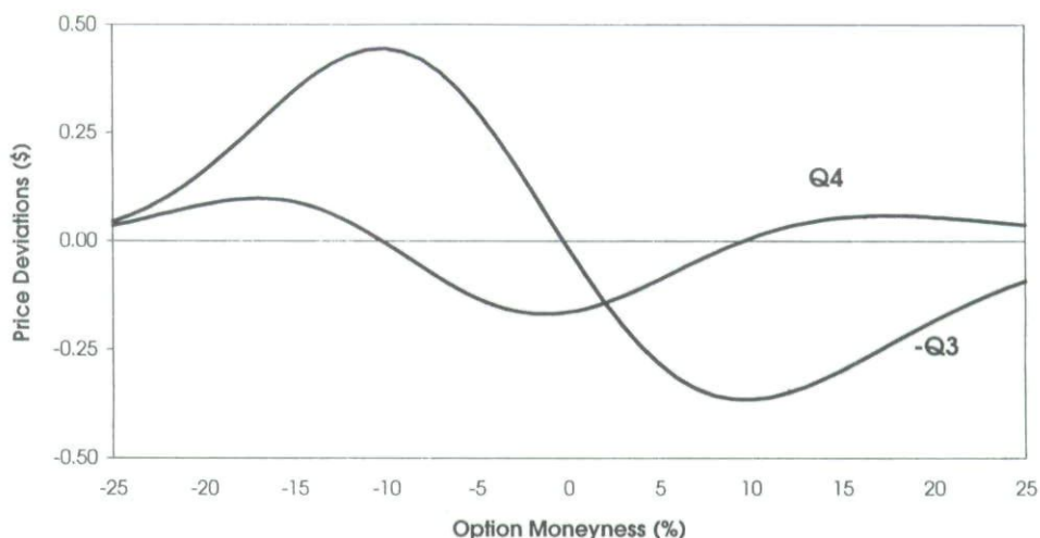
FIGURE 1 Skewness ( -Q_3 ) and kurtosis ( Q_4 ) deviations.
