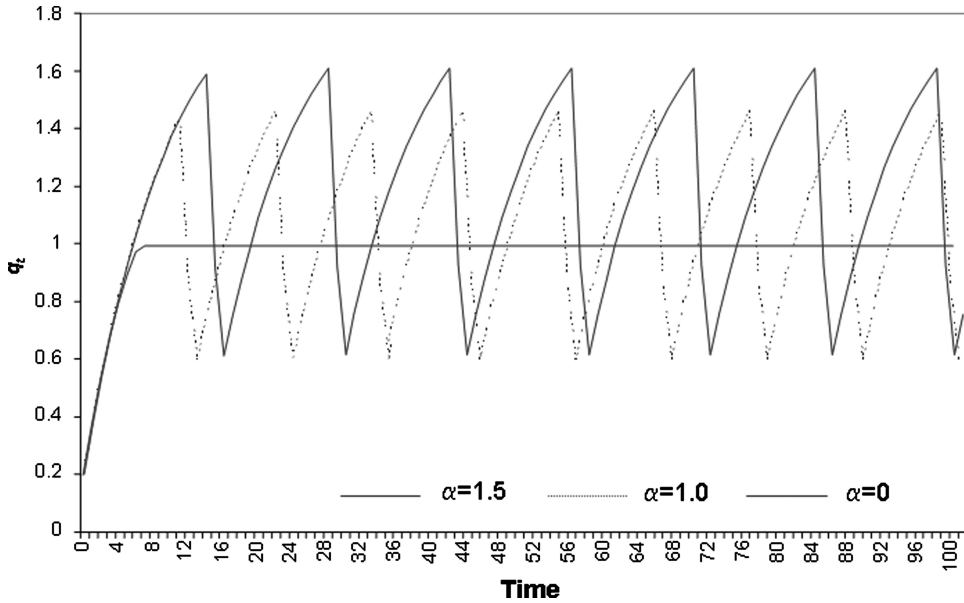
Figure 1. Deterministic cycles with constant demand flow. The parameter values are chosen as follows: Q = 2 , \gamma = 0.1 , A = 0.5 , v^a = v^s = v^m = 1 , \rho = 0.1 , and \delta = 1 . We then plot the evolution of q_t for three cases: (i) \alpha = 0 , (ii) \alpha = 1.0 , and (iii) \alpha = 1.5 .
