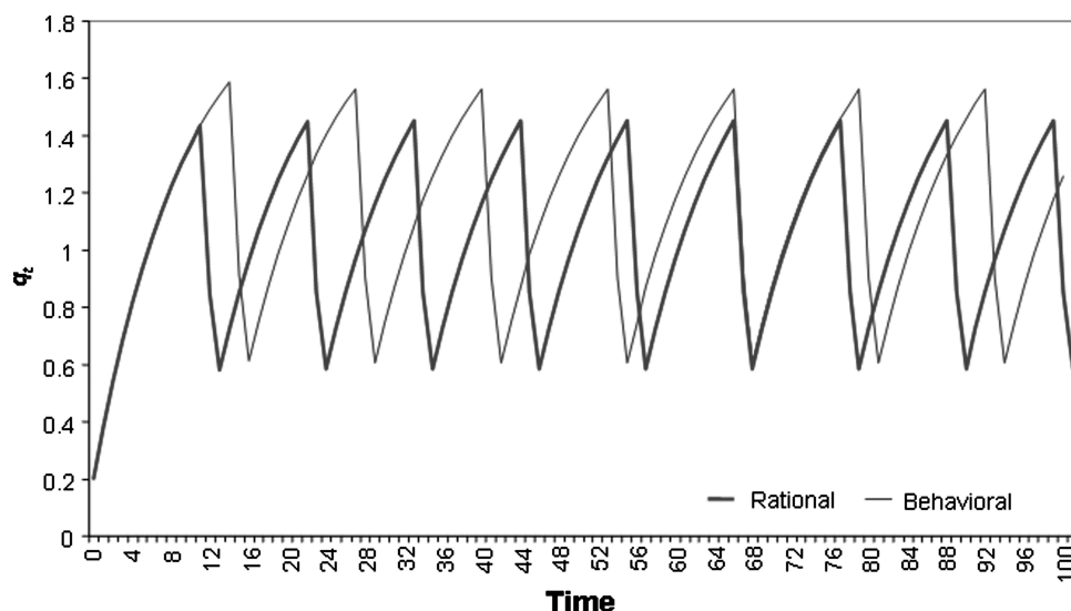
Figure 3. The effect of bounded rationality with constant demand flow. The parameter values are chosen as follows: Q = 2 , \gamma = 0.1 , A = 0.5 , v^a = v^s = v^m = 1 , \rho = 0.1 , and \delta = 1 . We then plot the evolution of q_t for two cases: (i) the case in which investors are fully rational, and (ii) the case in which investors are boundedly rational.
