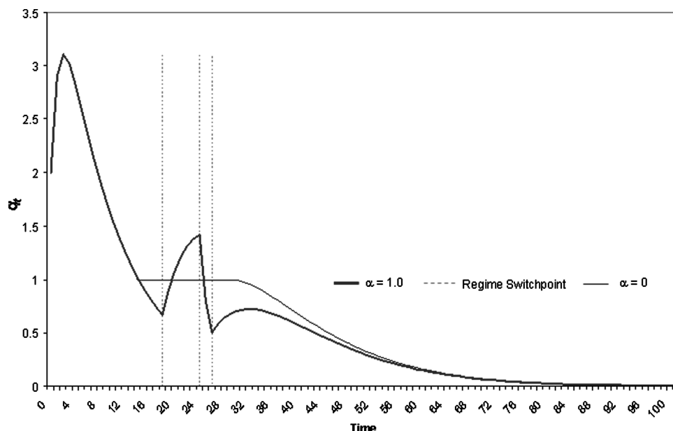
Figure 2. Nonmonotonic adjustment with shrinking demand flow. The parameter values are chosen as follows: Q_0 = 20 , \beta = 0.9 , \gamma = 0.1 , A = 0.5 , v^a = v^s = v^m = 1 , \rho = 0.1 , and \delta = 1 . We then plot the evolution of q_t for two cases: (i) \alpha = 0 and (ii) \alpha = 1.0 .
