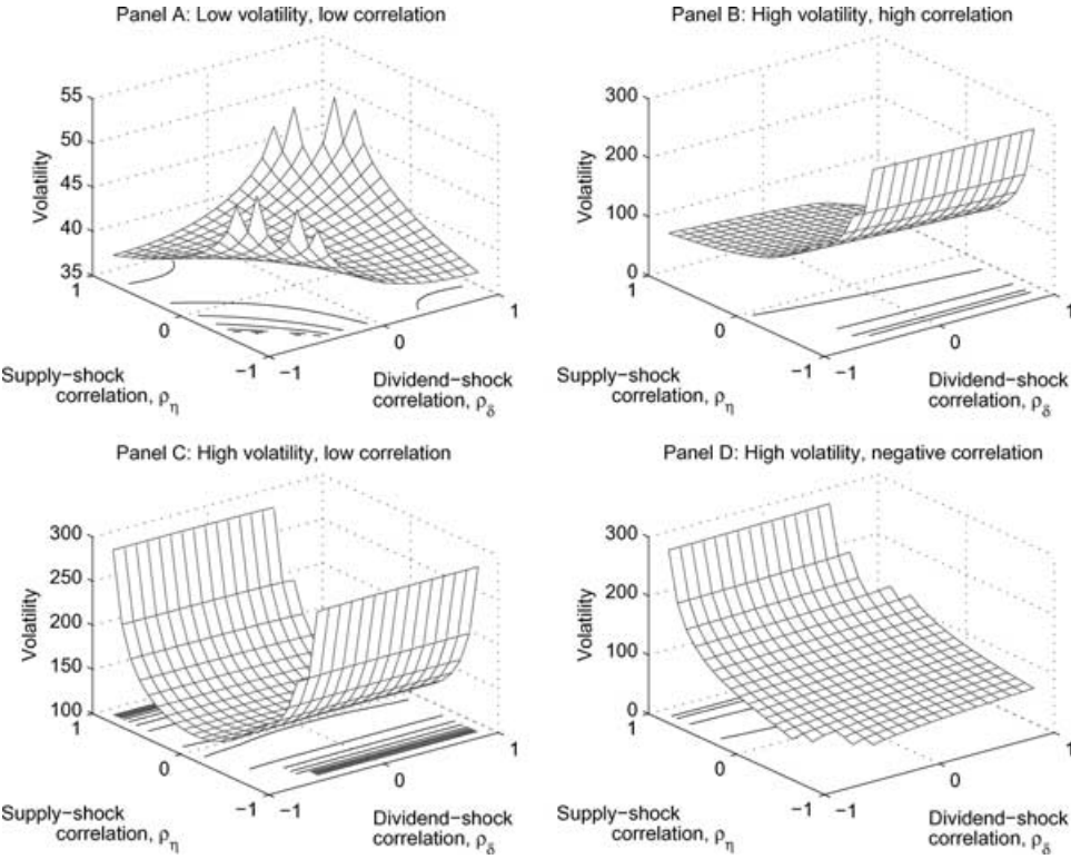
Figure 1. Volatility of individual stocks' price changes in a full information model with two symmetric securities. The panels represent the following four equilibria: Panel A—low volatility, low correlation; Panel B—high volatility, high correlation; Panel C—high volatility, low correlation; and Panel D—high volatility, negative correlation. Parameter values: \Sigma_\delta = 23.3^2 \begin{pmatrix} 1 & \rho_\delta \\ \rho_\delta & 1 \end{pmatrix} , \Sigma_\eta = 0.00499^2 \begin{pmatrix} 1 & \rho_\eta \\ \rho_\eta & 1 \end{pmatrix} , and r = 5\% per annum or 1.05^{10} - 1 .
