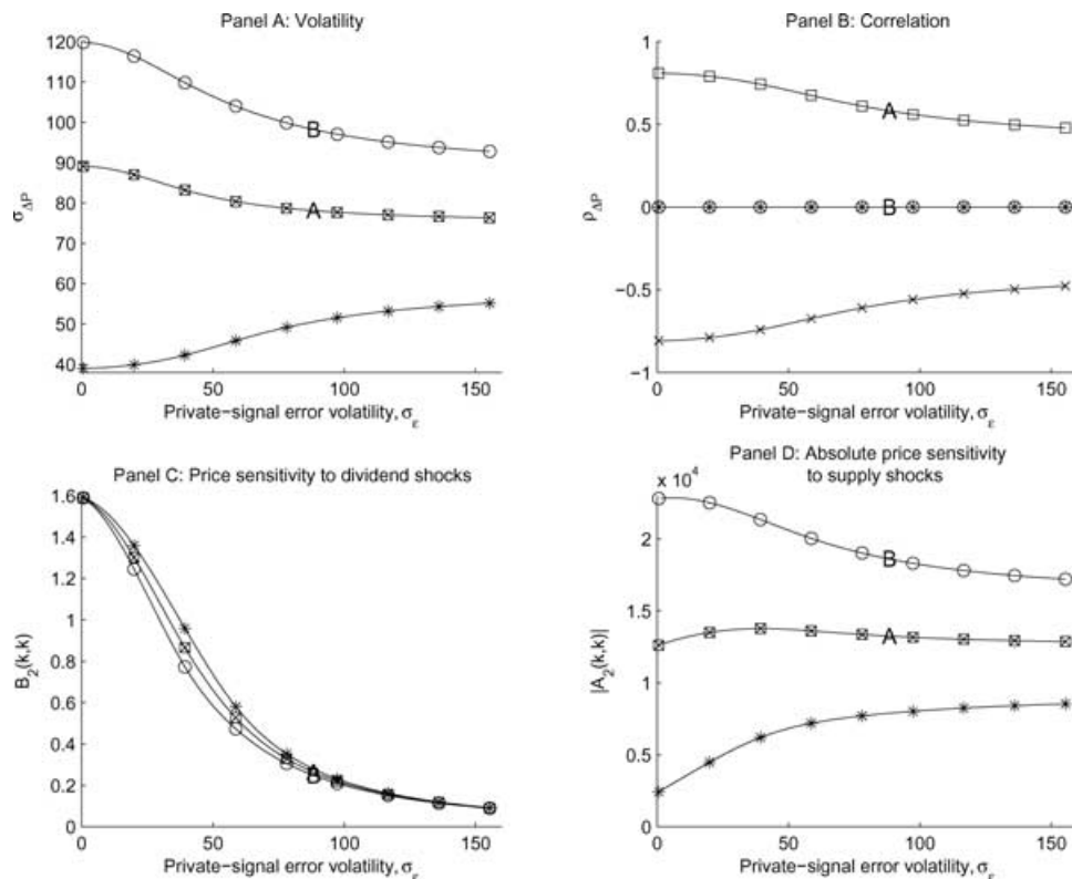
Figure 6. Price properties in a partial-information model with two symmetric securities. Panel A: Common volatility of individual stocks' price changes, \sigma_{AP} . Panel B: Cross-sectional correlation between the two stocks' price changes, \rho_{AP} . Panel C: A stock's price sensitivity to its own future dividend shock, B_2(k, k) . Panel D: A stock's absolute price sensitivity to its own supply shock, |A_2(k, k)| . The markers represent the following equilibria: stars—low volatility, low correlation; squares—high volatility, high correlation; circles—high volatility, low correlation; and crosses—high volatility, negative correlation. Points A and B give Shiller's (1981b) aggregate volatility estimate, 69.4. Parameter values: \Sigma_\delta = 23.3^2 I , \Sigma_\eta = 0.00499^2 I , \bar{\Sigma}_\epsilon = \sigma_\epsilon^2 I , \Sigma_\zeta^{1/2} = 4\Sigma_\eta^{1/2} , and r = 5\% per annum or 1.05^{10} - 1 .
