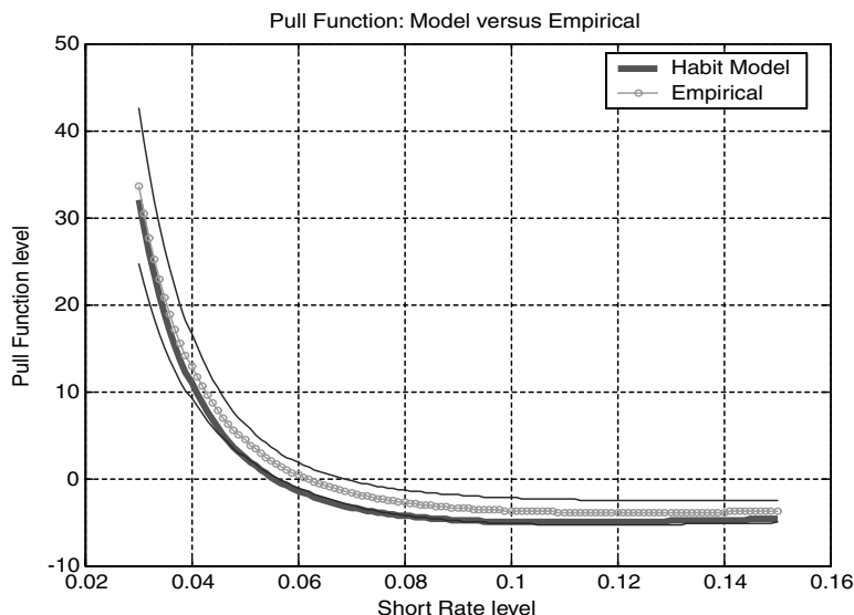
Figure 3. Pull function. The plots shows the empirical pull function based on the flexible semi-parametric approach by Conley et al. (1997), which uses a flexible parameterization of the local volatility \sigma(r_t) = \sum_{i=0}^{\gamma} \sigma_i r_t^i , and the habit model-implied pull function. The two thin solid lines are the 95% confidence bounds around the empirical functions.
