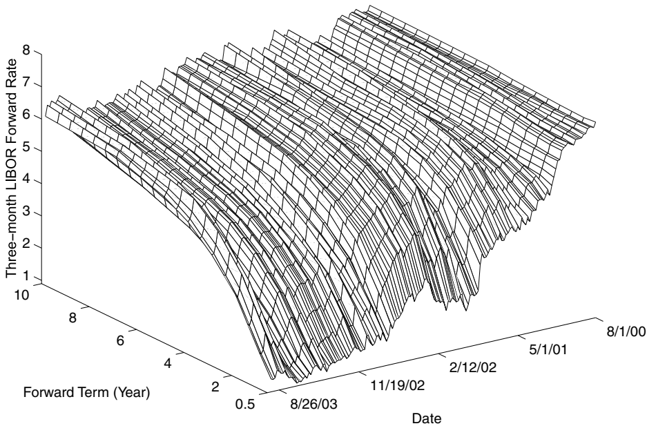
Figure 1. Term structure of 3-month LIBOR forward rates between August 1, 2000 and September 23, 2003.
