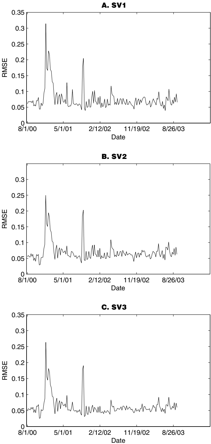
Figure 6. The RMSEs from SV models between August 1, 2000 and September 23, 2003.
