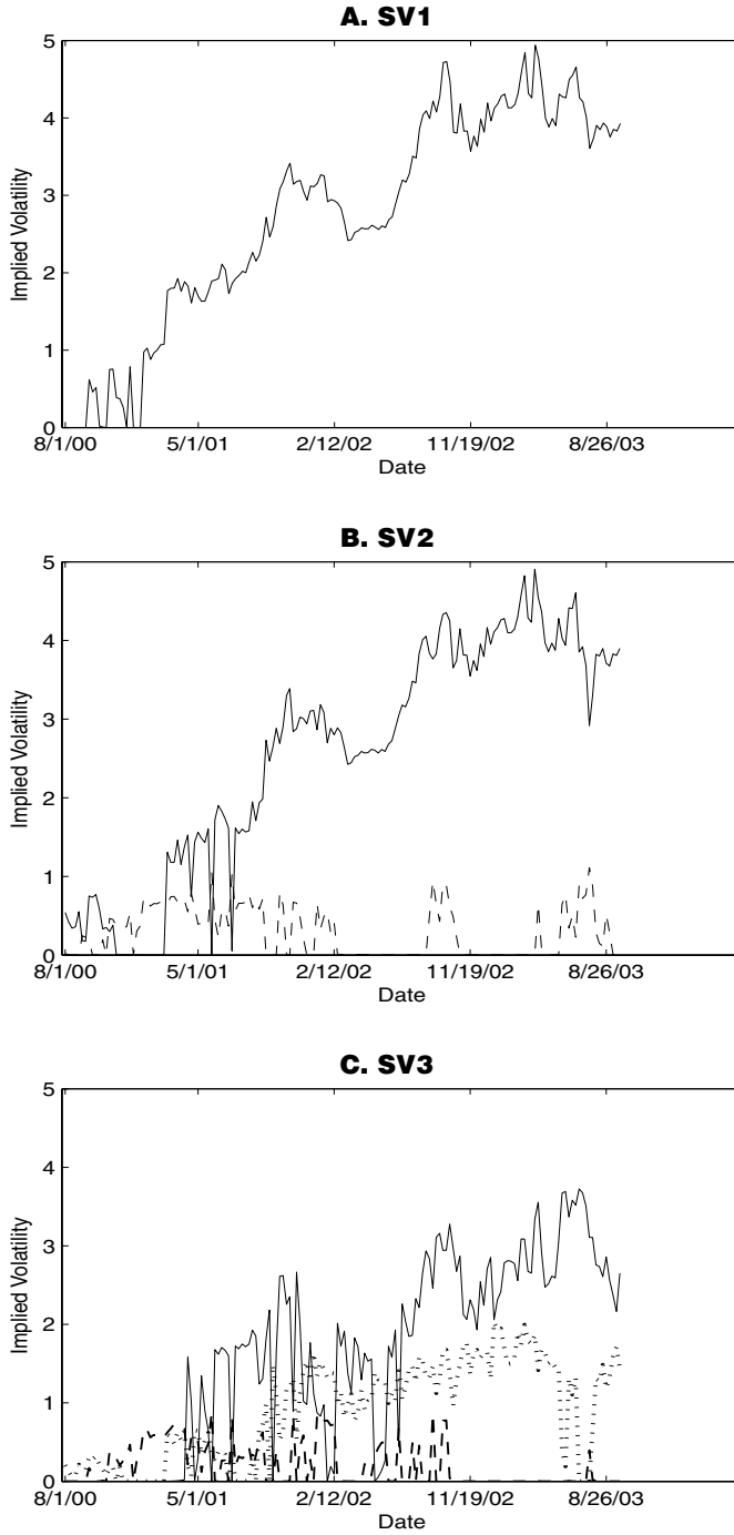
Figure 5. The implied volatilities from SV models between August 1, 2000 and September 23, 2003 (solid: first factor; dashed: second factor; dotted: third factor).
