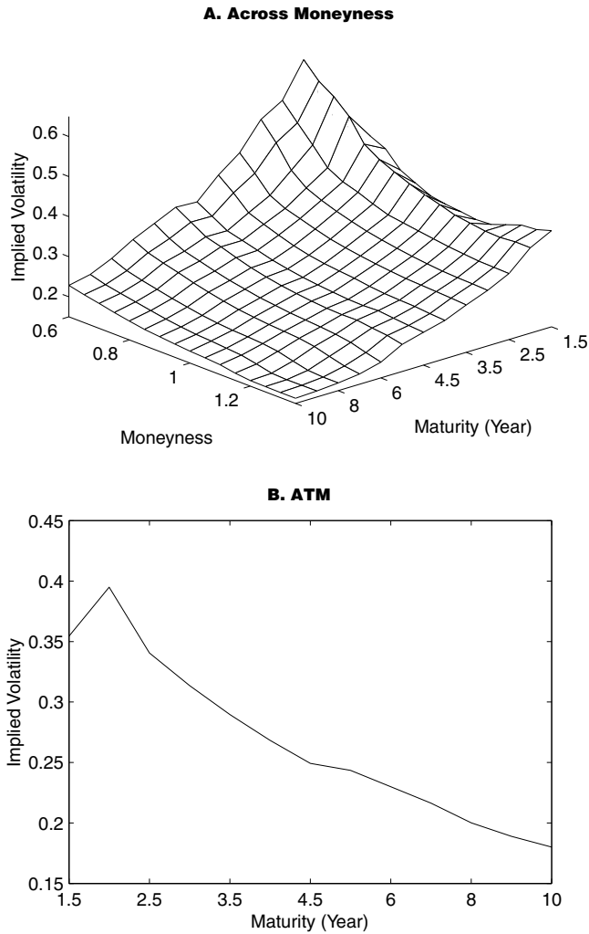
Figure 2. Average Black's implied volatilities of difference caps between August 1, 2000 and September 23, 2003.
