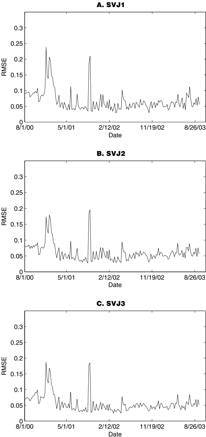
Figure 8. The RMSEs from SVJ models between August 1, 2000 and September 23, 2003.
