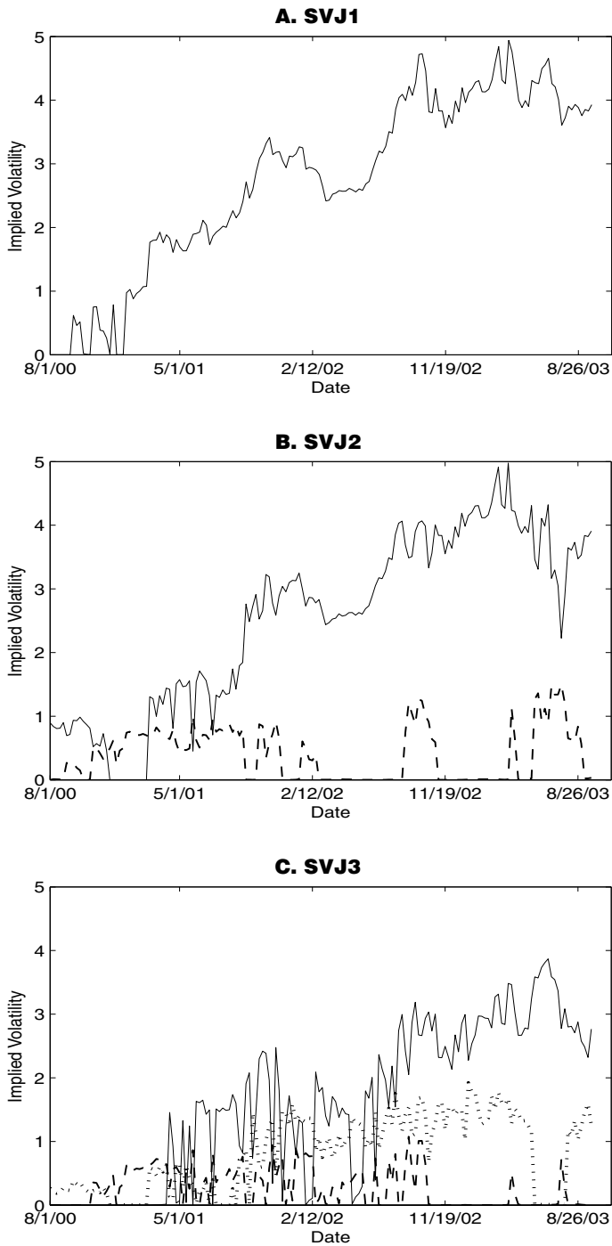
Figure 7. The implied volatilities from SVJ models between August 1, 2000 and September 23, 2003 (solid: first factor; dashed: second factor; dotted: third factor).
