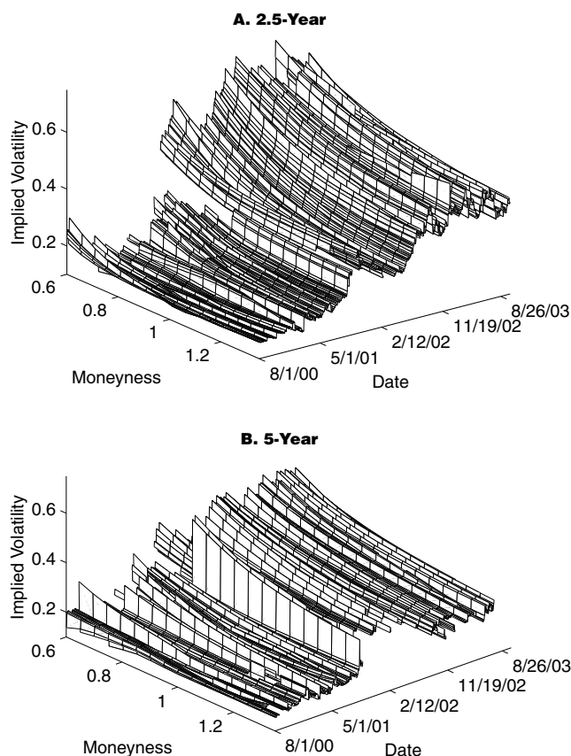
Figure 3. Black's implied volatilities of 2.5-, 5-, and 8-year difference caps between August 1, 2000 and September 23, 2003.
