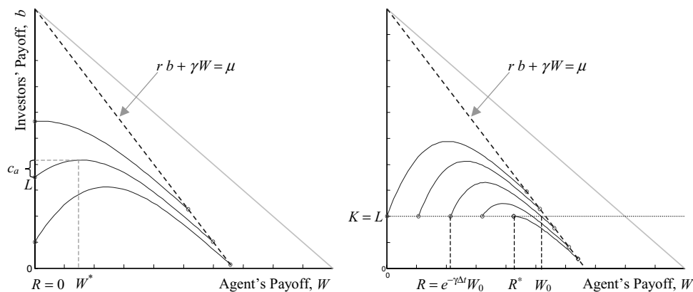
Figure 7. Determining L or R endogenously. The left panel considers the case in which the agent can be fired and replaced at cost c_a , so that L = b(W^*) - c_a . The right panel considers the case in which the agent can quit and raise capital K (in the example, K = L ) to start a new firm with delay \Delta t , so that R = e^{-\gamma \Delta t} W_0 .
