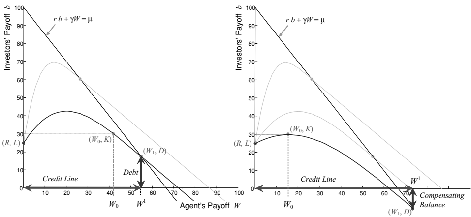
Figure 3. The optimal contract with medium and high volatility. For \sigma = 12.5 and \sigma = 19.07 .
