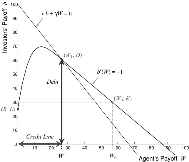
Figure 2. The optimal contract with low volatility. For L = 25 , R = 0 , \mu = 10 , \sigma = 5 , r = 10\% , \gamma = 15\% , \lambda = 1 , K = 30 .
