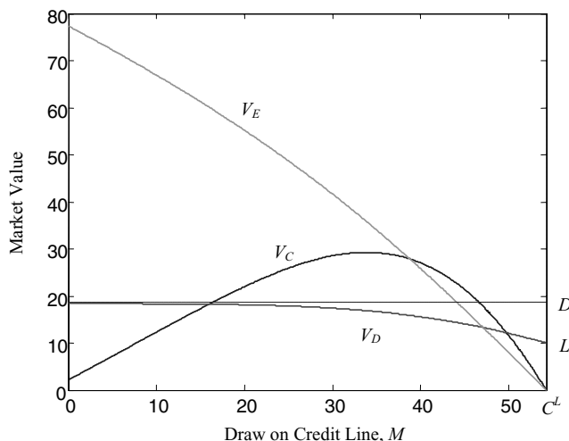
Figure 5. Market values of securities. For \mu = 10 , \sigma = 10 , \lambda = 50\% , r = 10\% , \gamma = 15\% , L = 10 , R = 0 .
