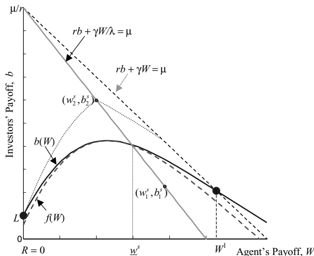
Figure 6. The optimal contract with hidden effort. If A is sufficiently large so that (w^s, b^s) is below the curve f(W) , then high effort is optimal and the optimal contract is the same as in the cash flow diversion model of Section I.
