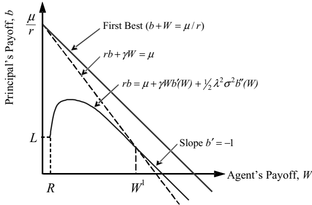
Figure 1. The principal's value function b(W) . The principal's value function starts at (R, L) , and obeys the differential equation (15) until the point W^1 , and then continues with slope -1 .
