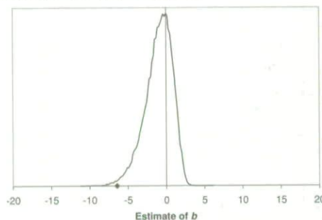
Figure 1. Pseudo market timing and predictive regressions based on equity issuance. We simulate 50,000 estimates from the following system of equations:
