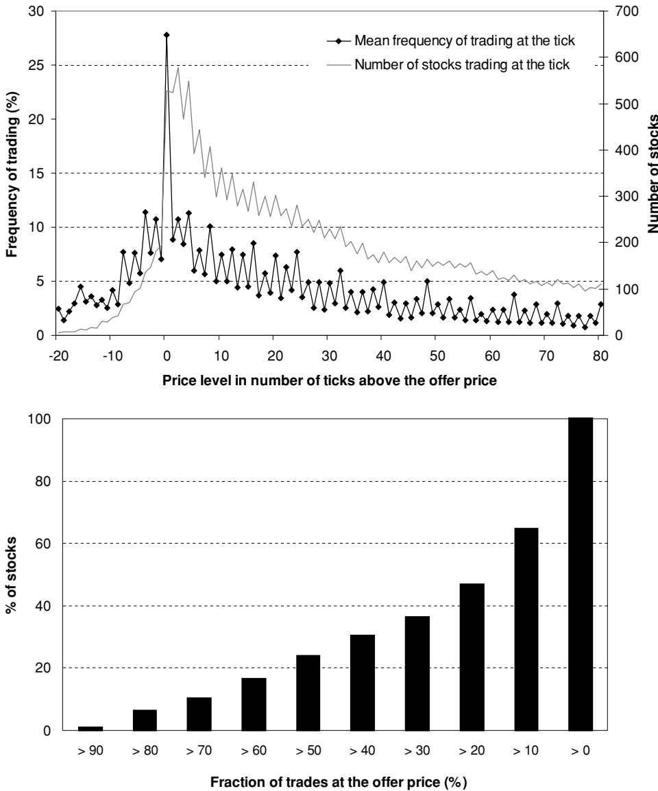
Figure 1. Frequency of trading at and around the offer price on day 1. The top figure compares the frequency of trading on day 1 at various price levels around the offer price. Price levels are measured in the number of ticks above the offer price (tick = $0.125). The thin line depicts the number of stocks that trade at least once at a given price level on day 1. The bold line shows the average fraction of trades at each price level for stocks that trade at least once at that price. The bottom figure focuses on 527 stocks that trade at least once at the offer price on day 1. It shows a histogram of percent of all first-day trades executed at the offer price. For example, 65% of the 527 stocks trade at least 10% of time at the offer price.
