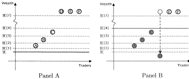
Figure 4. Systemic risk in setting with endogenous distress. This figure shows the wealth levels of traders A, ..., E and several survival hurdles W(I^d) , that is, the wealth necessary to survive if the market believes that I^d traders will be in distress. In Panel A, traders' wealth levels are high enough that all traders survive in the unique equilibrium. In Panel B, trader D is in distress because of a wealth shock. This leads to predatory trading which can drag traders A, B, and C into distress too.
