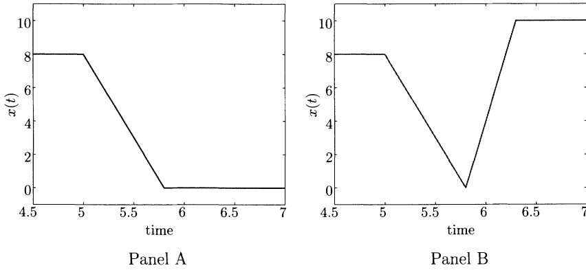
Figure 1. Holdings of distressed trader (Panel A) and of single predator (Panel B). Starting with an initial holding of x^i(t_0) = 8 , both traders sell at maximum intensity of A/2 = 10 from t_0 = 5 until t_0 + \frac{x(t_0)}{A/2} = 5.8 . By then, the distressed trader has completed his liquidation and subsequently the predator buys back shares.
