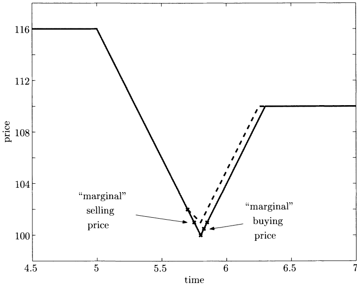
Figure 2. Price dynamics with single predator. The price falls as the distressed trader and the predator sell from time 5 to time 5.8, and rebounds as the predator buys back. The predation leads to price overshooting and a low liquidation value for the distressed trader—the market is illiquid when the distressed trader needs liquidity. The dotted line represents the hypothetical price dynamics if the predator sells one share less, that is, if only the distressed trader sells from time 5.7 to time 5.8. This hypothetical behavior is not optimal since the last “marginal” share can be sold at an average price of 101.00 and then can be bought back cheaper at 100.50.
